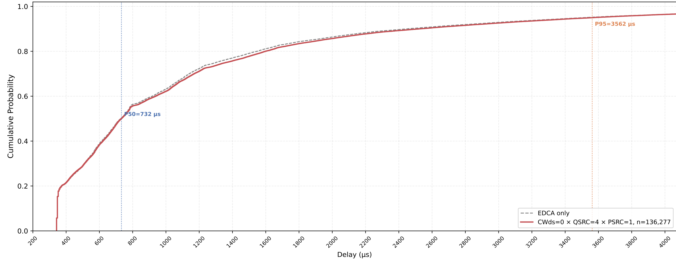
Legacy STA VO Delay CDF — CWds=0 × QSRC=4 × PSRC=1 nSta=30, nPedca=5, 0.5Mbps, avg of 10 runs
