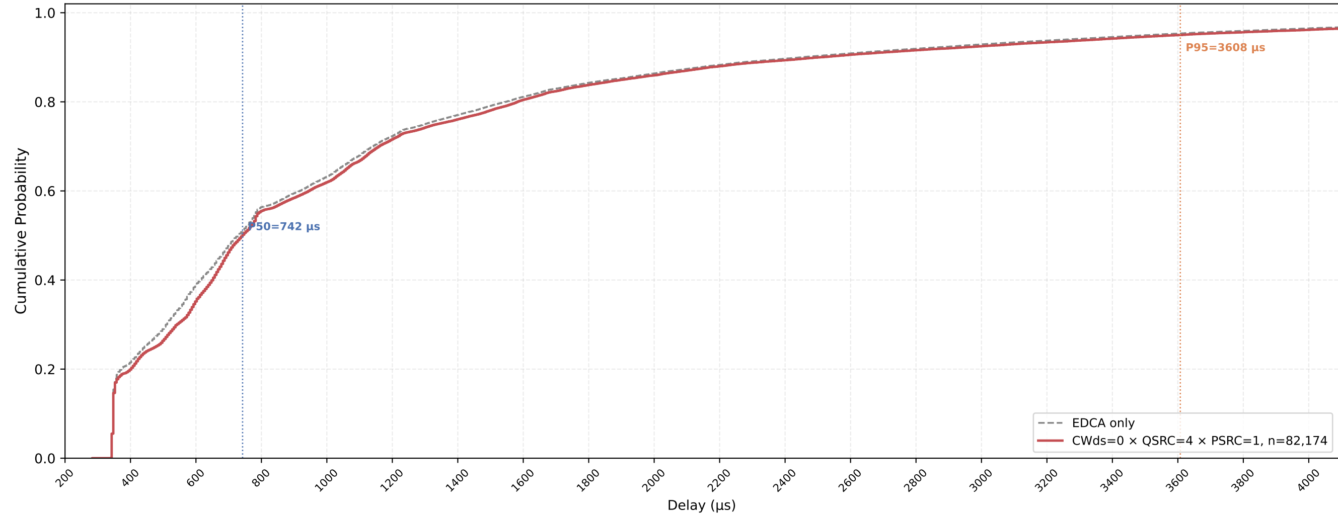
Legacy STA VO Delay CDF — CWds=0 × QSRC=4 × PSRC=1 nSta=30, nPedca=15, 0.5Mbps, avg of 10 runs
