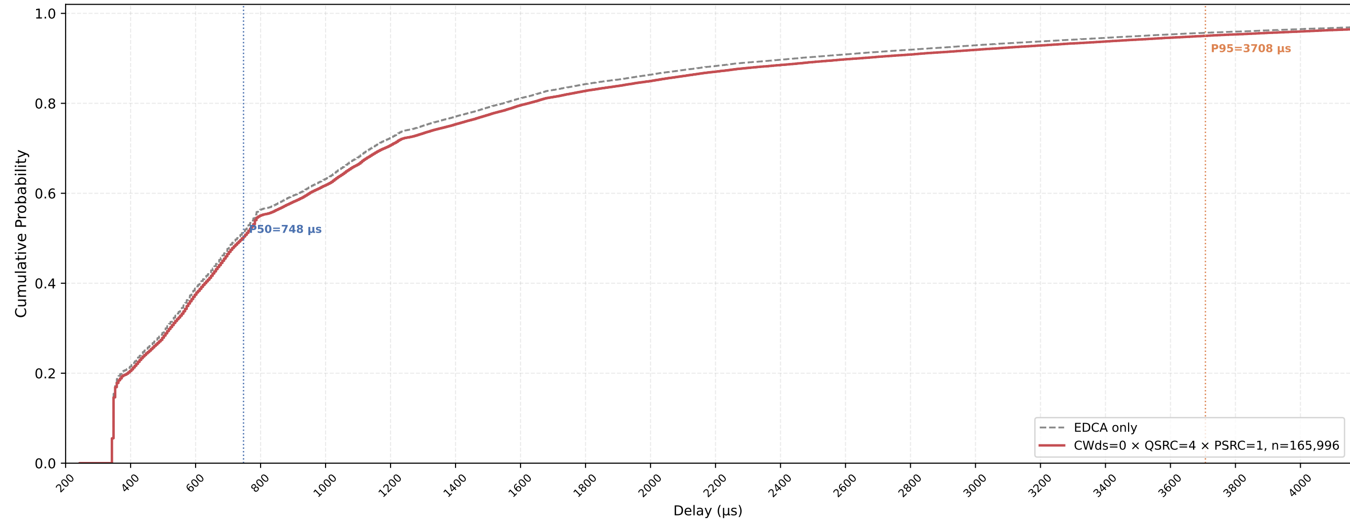
P-EDCA STA VO Delay CDF — CWds=0 × QSRC=4 × PSRC=1 nSta=30, nPedca=30, 0.5Mbps, avg of 10 runs
