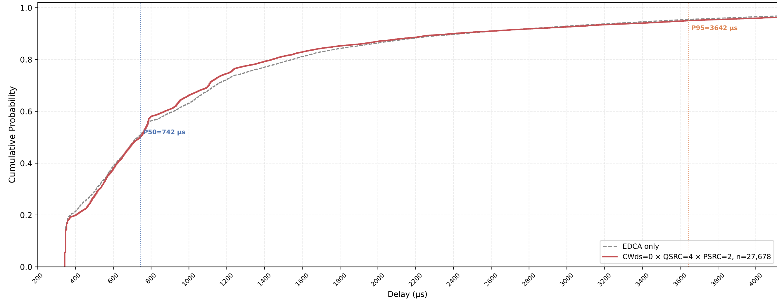
P-EDCA STA VO Delay CDF — CWds=0 × QSRC=4 × PSRC=2 nSta=30, nPedca=5, 0.5Mbps, avg of 10 runs
