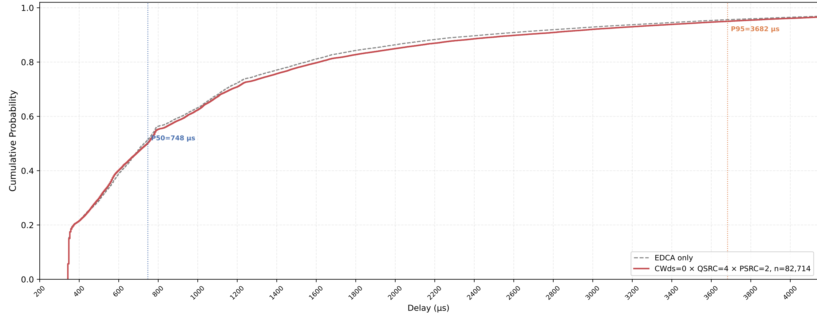
P-EDCA STA VO Delay CDF — CWds=0 × QSRC=4 × PSRC=2 nSta=30, nPedca=15, 0.5Mbps, avg of 10 runs
