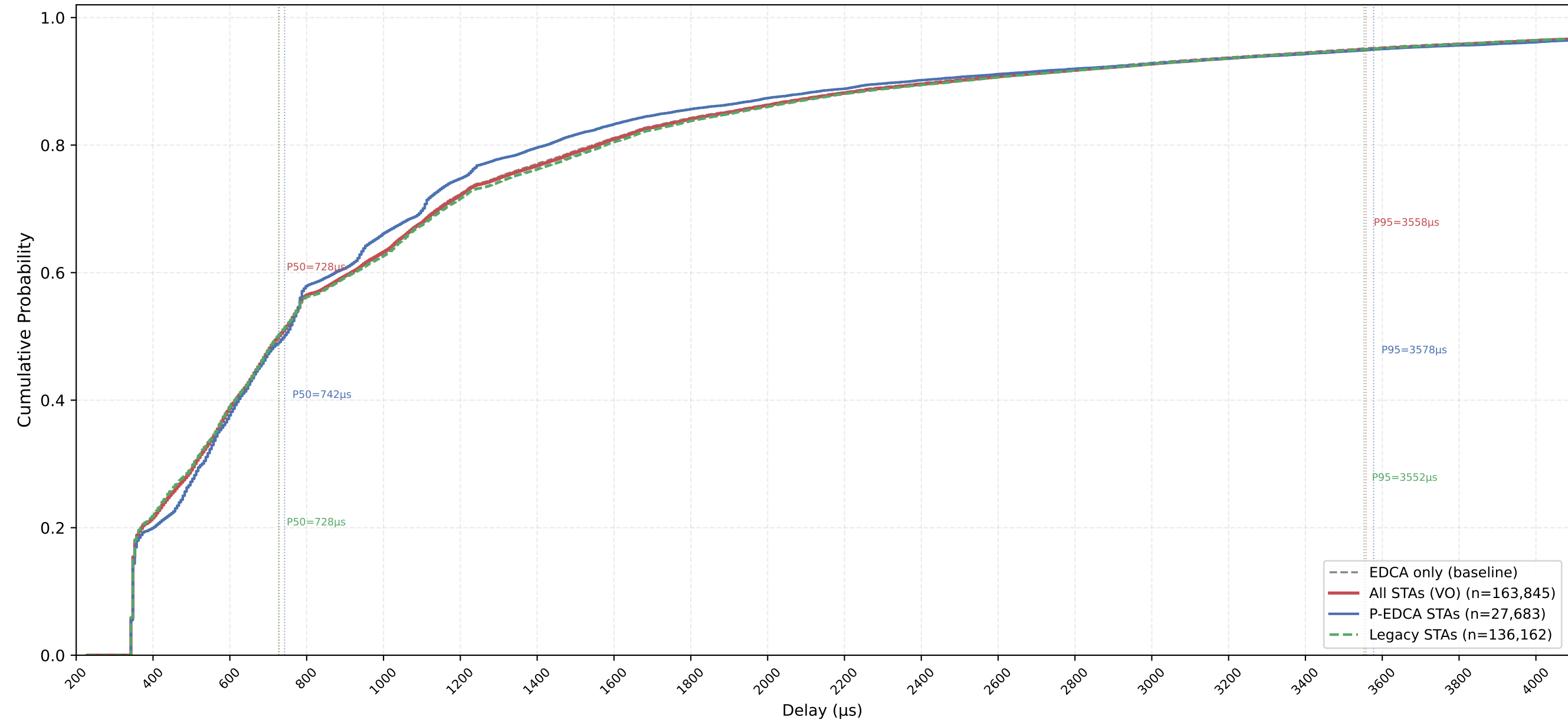
VO Delay CDF — P-EDCA / Legacy / All | CWds=0 × QSRC=4 × PSRC=3 nSta=30, nPedca=5/30, 0.5Mbps, avg of 10 runs
