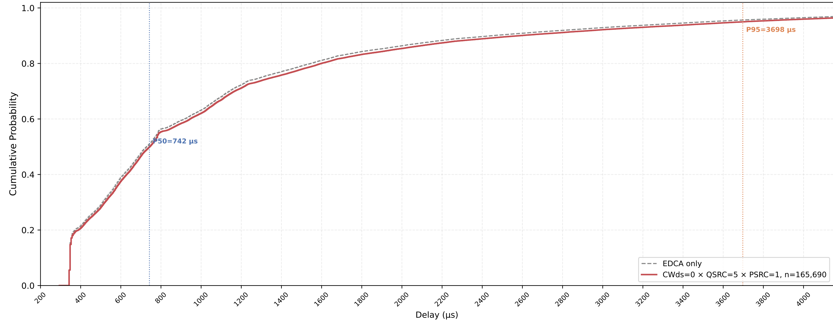
VO (all STAs) Delay CDF — CWds=0 × QSRC=5 × PSRC=1 nSta=30, nPedca=30, 0.5Mbps, avg of 10 runs
