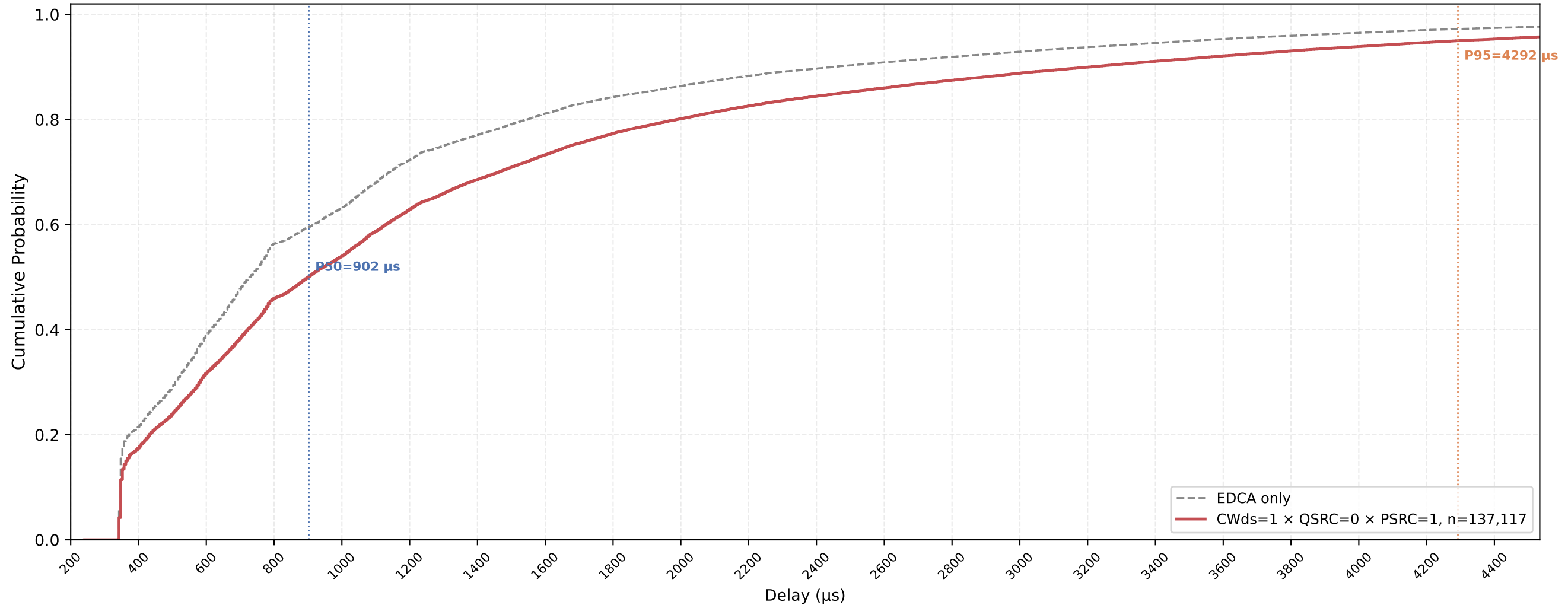
Legacy STA VO Delay CDF — CWds=1 × QSRC=0 × PSRC=1 nSta=30, nPedca=5, 0.5Mbps, avg of 10 runs
