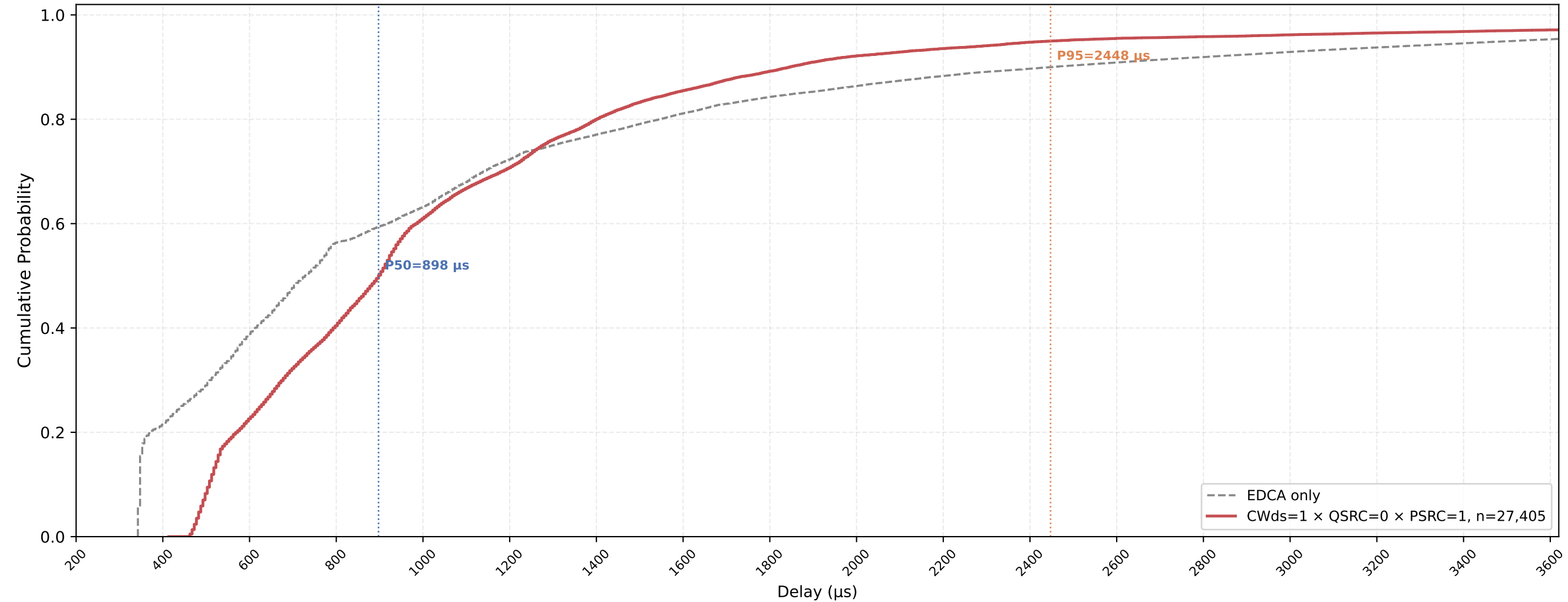
P-EDCA STA VO Delay CDF — CWds=1 × QSRC=0 × PSRC=1 nSta=30, nPedca=5, 0.5Mbps, avg of 10 runs
