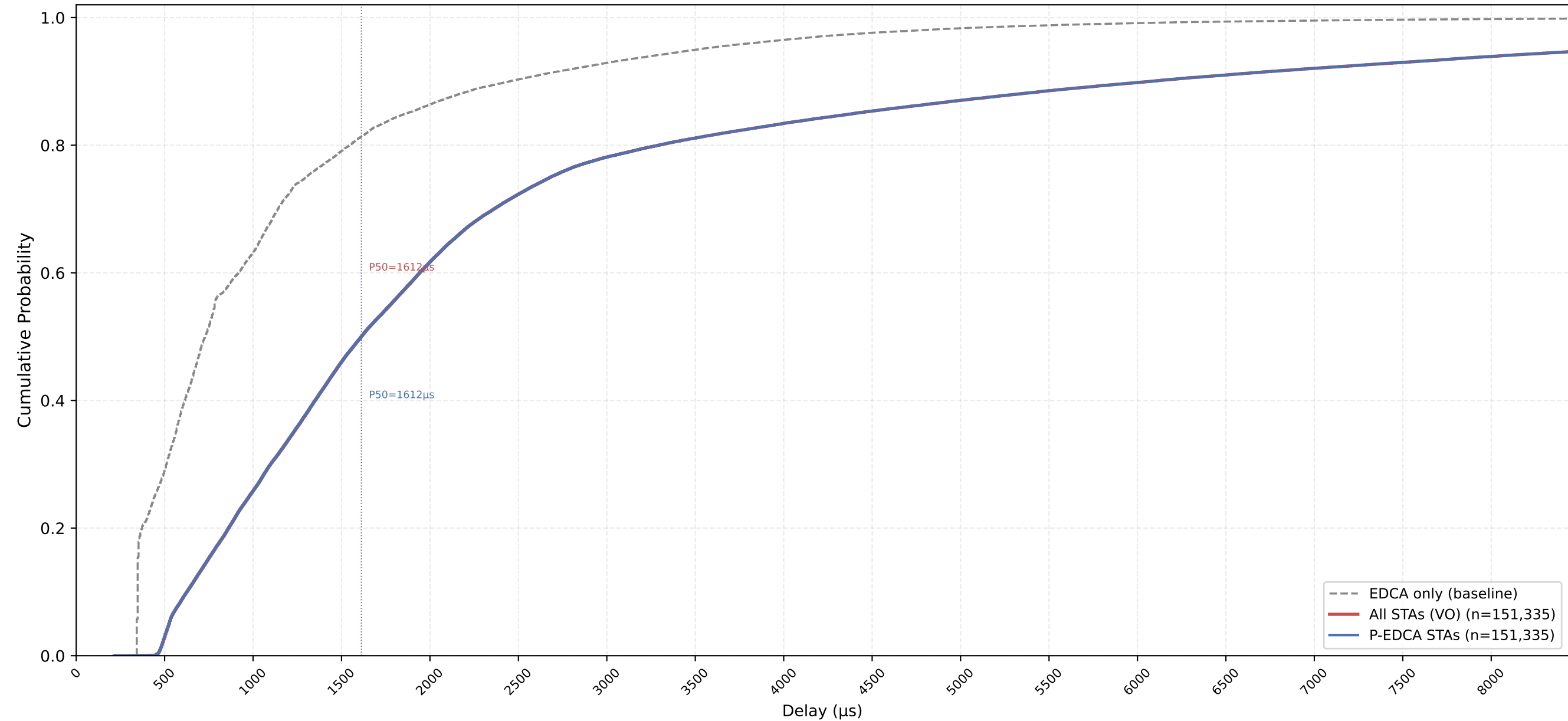
VO Delay CDF — P-EDCA / Legacy / All | CWds=1 × QSRC=0 × PSRC=2 nSta=30, nPedca=30/30, 0.5Mbps, avg of 10 runs
