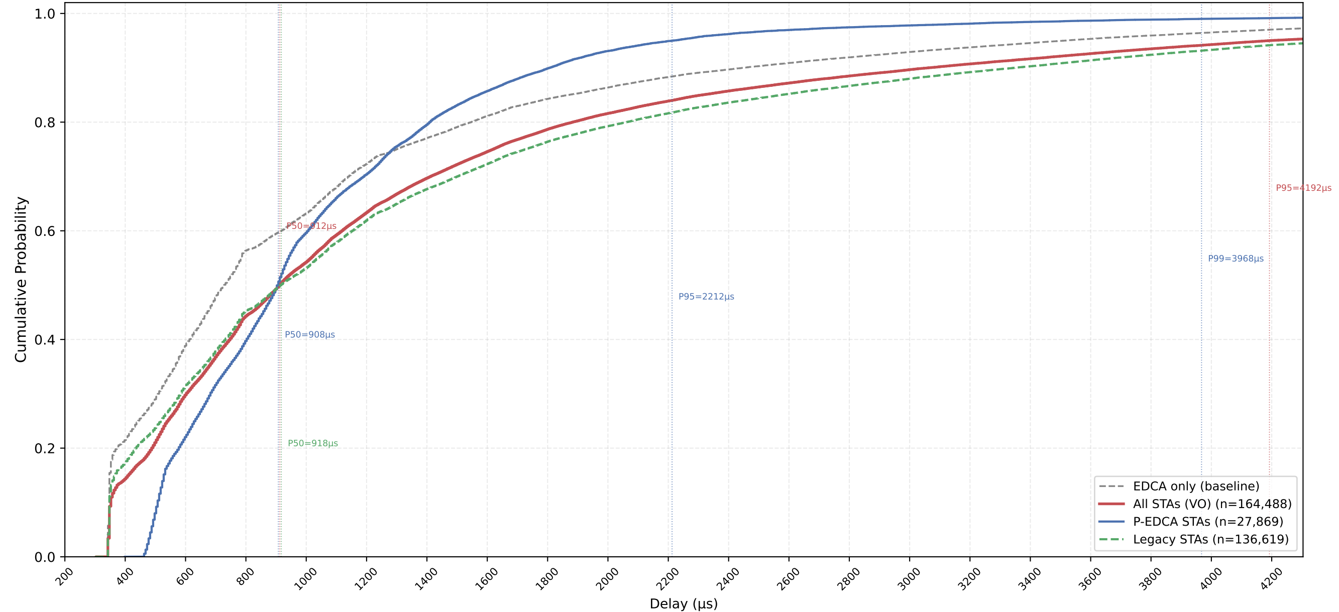
VO Delay CDF — P-EDCA / Legacy / All | CWds=1 × QSRC=0 × PSRC=3 nSta=30, nPedca=5/30, 0.5Mbps, avg of 10 runs
