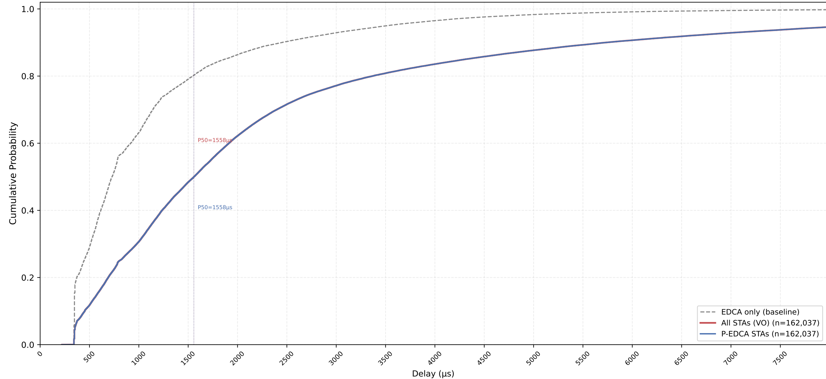
VO Delay CDF — P-EDCA / Legacy / All | CWds=1 × QSRC=1 × PSRC=2 nSta=30, nPedca=30/30, 0.5Mbps, avg of 10 runs
