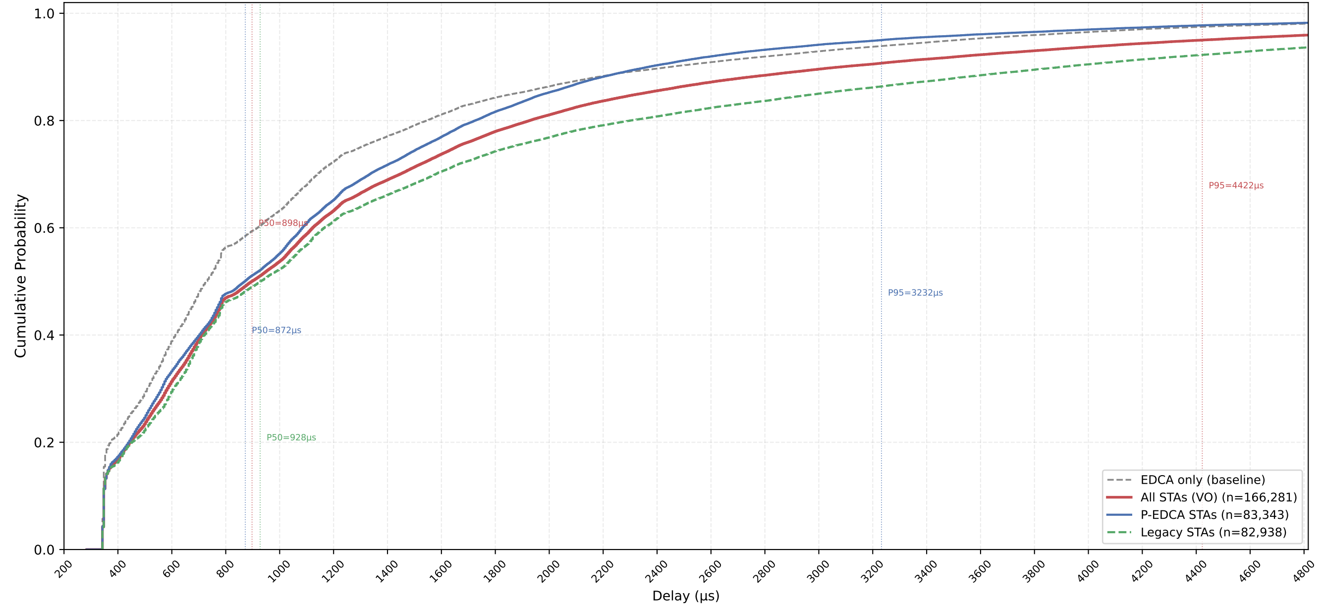
VO Delay CDF — P-EDCA / Legacy / All | CWds=1 × QSRC=1 × PSRC=3 nSta=30, nPedca=15/30, 0.5Mbps, avg of 10 runs
