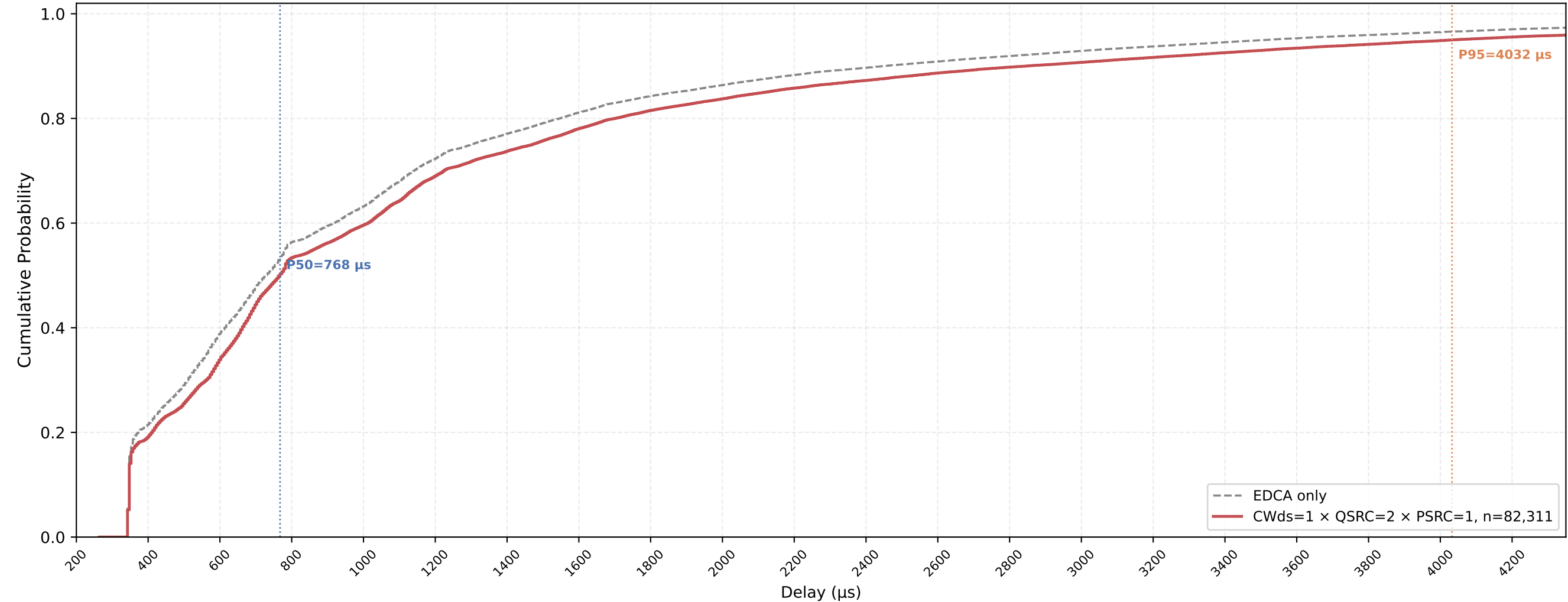
Legacy STA VO Delay CDF — CWds=1 × QSRC=2 × PSRC=1 nSta=30, nPedca=15, 0.5Mbps, avg of 10 runs
