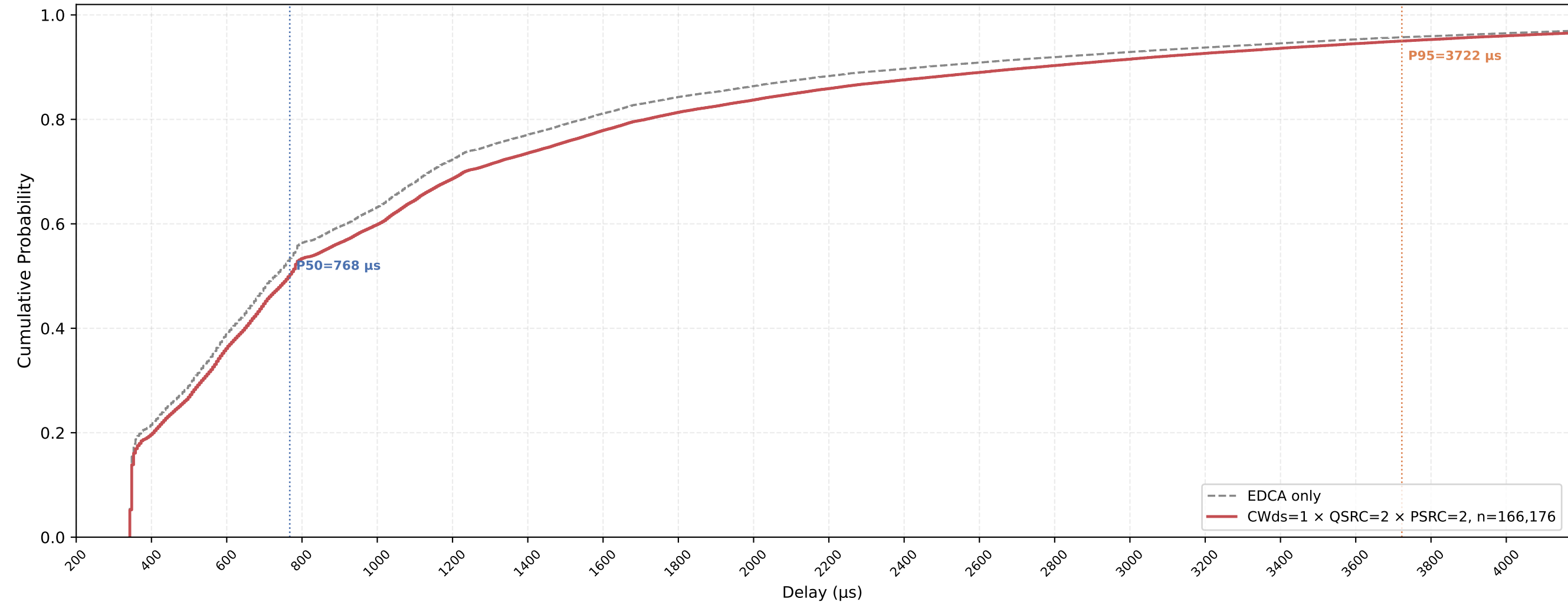
VO (all STAs) Delay CDF — CWds=1 × QSRC=2 × PSRC=2 nSta=30, nPedca=15, 0.5Mbps, avg of 10 runs
