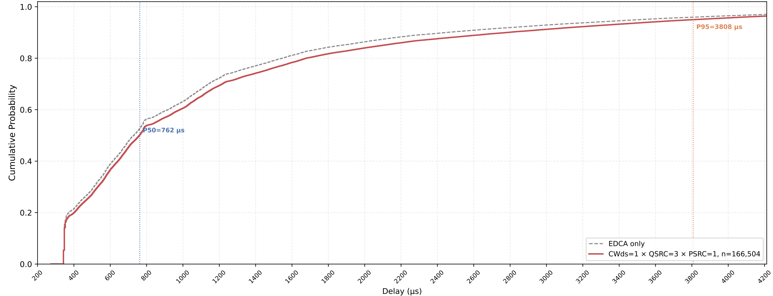
P-EDCA STA VO Delay CDF — CWds=1 × QSRC=3 × PSRC=1 nSta=30, nPedca=30, 0.5Mbps, avg of 10 runs
