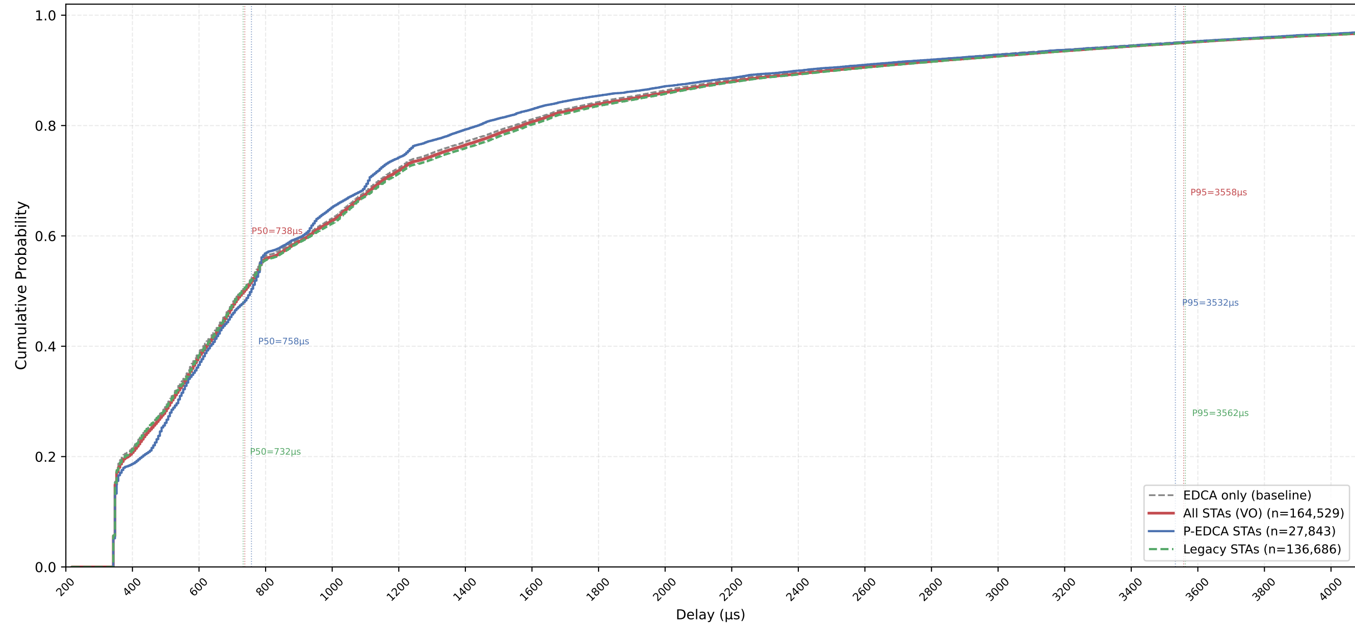
VO Delay CDF — P-EDCA / Legacy / All | CWds=1 × QSRC=3 × PSRC=2 nSta=30, nPedca=5/30, 0.5Mbps, avg of 10 runs
