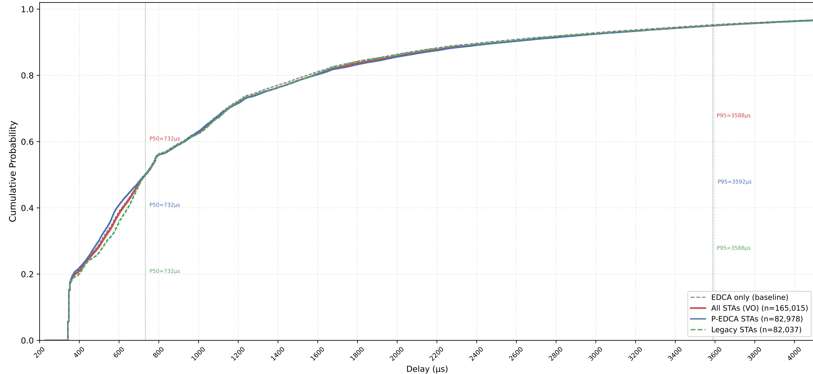
VO Delay CDF — P-EDCA / Legacy / All | CWds=1 × QSRC=4 × PSRC=1 nSta=30, nPedca=15/30, 0.5Mbps, avg of 10 runs
