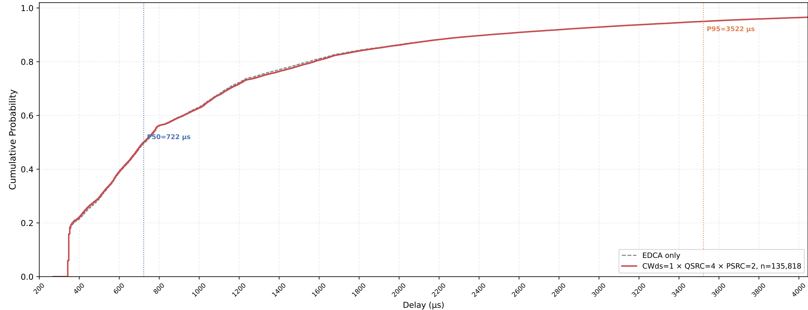
Legacy STA VO Delay CDF — CWds=1 × QSRC=4 × PSRC=2 nSta=30, nPedca=5, 0.5Mbps, avg of 10 runs
