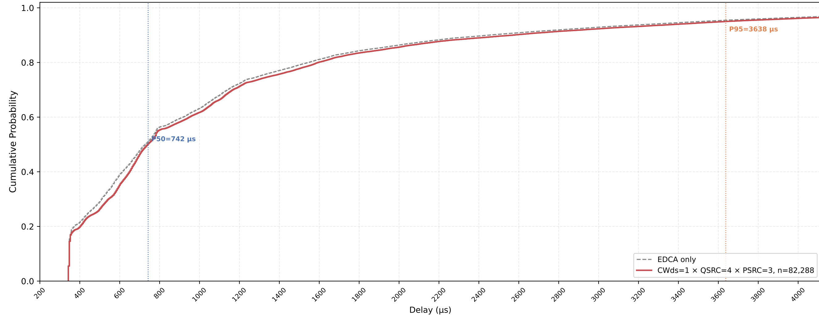
Legacy STA VO Delay CDF — CWds=1 × QSRC=4 × PSRC=3 nSta=30, nPedca=15, 0.5Mbps, avg of 10 runs
