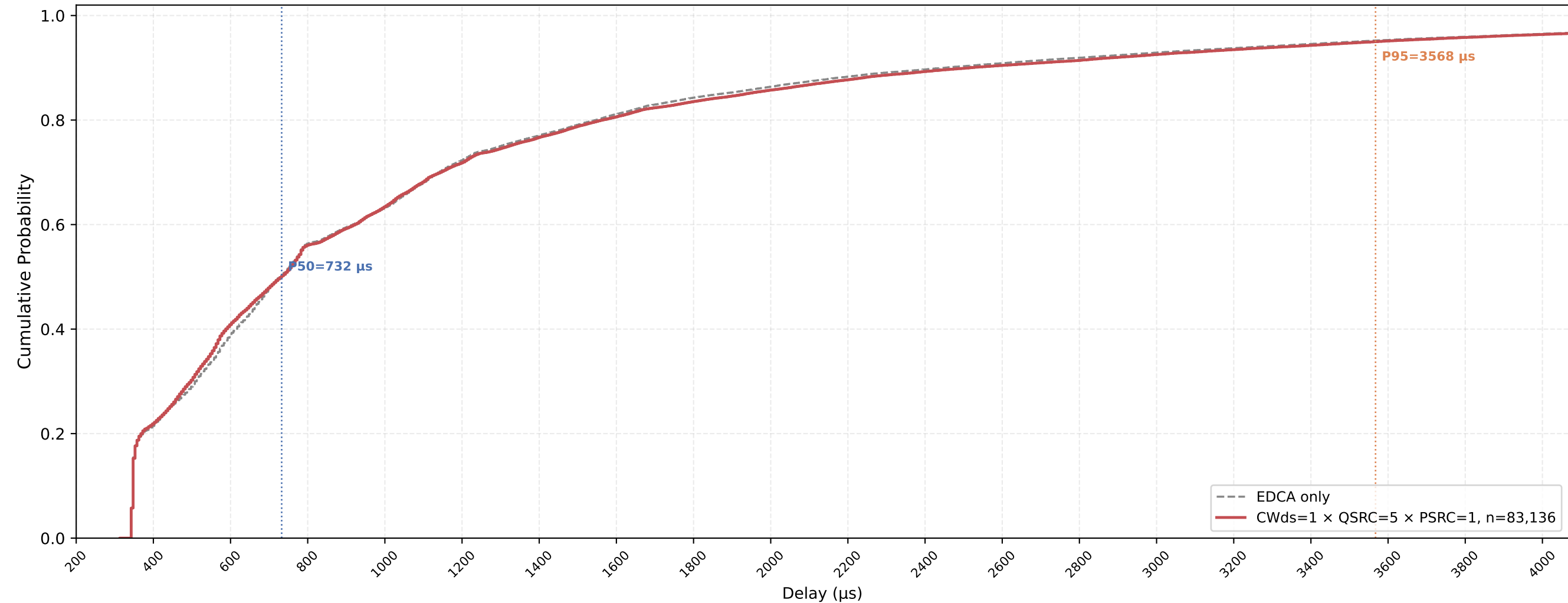
P-EDCA STA VO Delay CDF — CWds=1 × QSRC=5 × PSRC=1 nSta=30, nPedca=15, 0.5Mbps, avg of 10 runs
