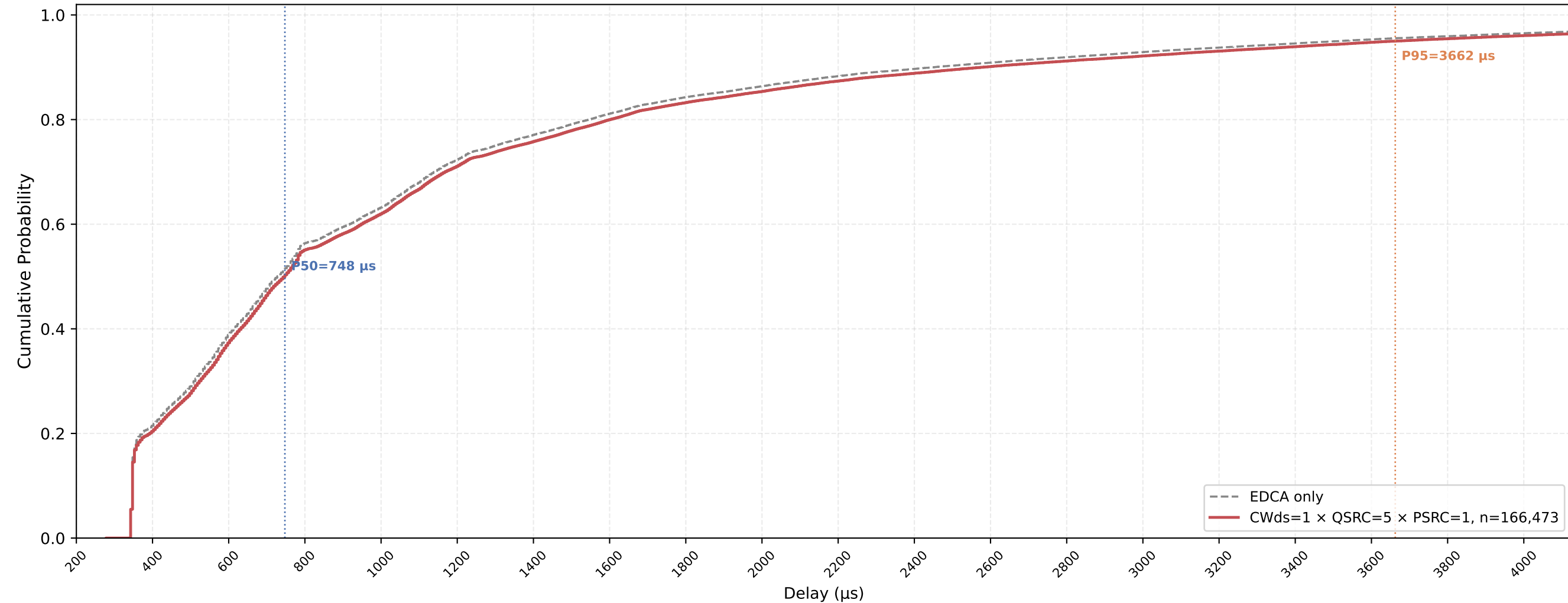
VO (all STAs) Delay CDF — CWds=1 × QSRC=5 × PSRC=1 nSta=30, nPedca=30, 0.5Mbps, avg of 10 runs
