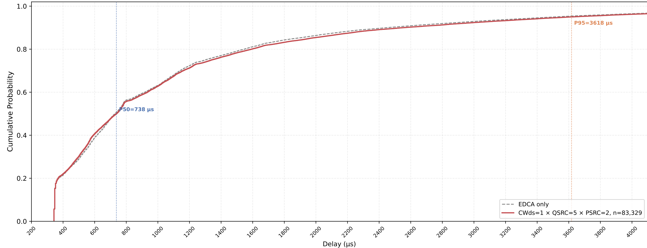
P-EDCA STA VO Delay CDF — CWds=1 × QSRC=5 × PSRC=2 nSta=30, nPedca=15, 0.5Mbps, avg of 10 runs
