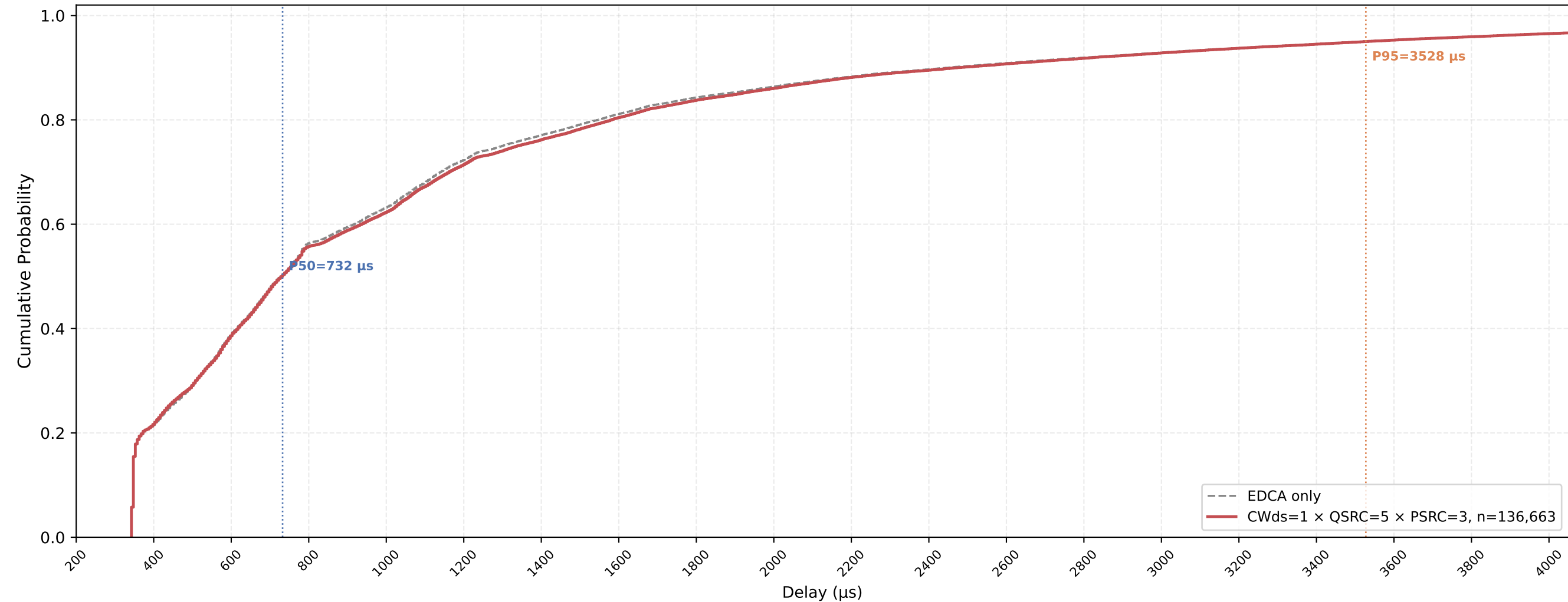
Legacy STA VO Delay CDF — CWds=1 × QSRC=5 × PSRC=3 nSta=30, nPedca=5, 0.5Mbps, avg of 10 runs
