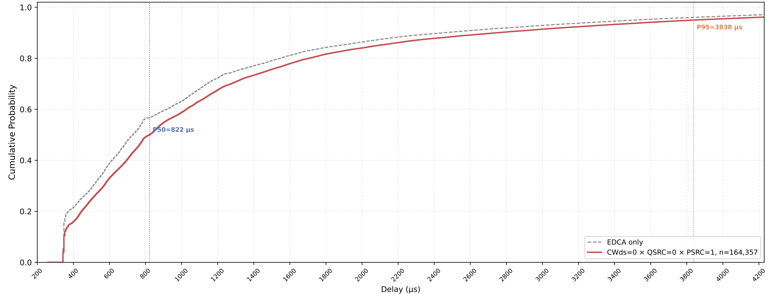
VO (all STAs) Delay CDF — CWds=0 × QSRC=0 × PSRC=1 nSta=30, nPedca=5, 0.5Mbps, avg of 10 runs
