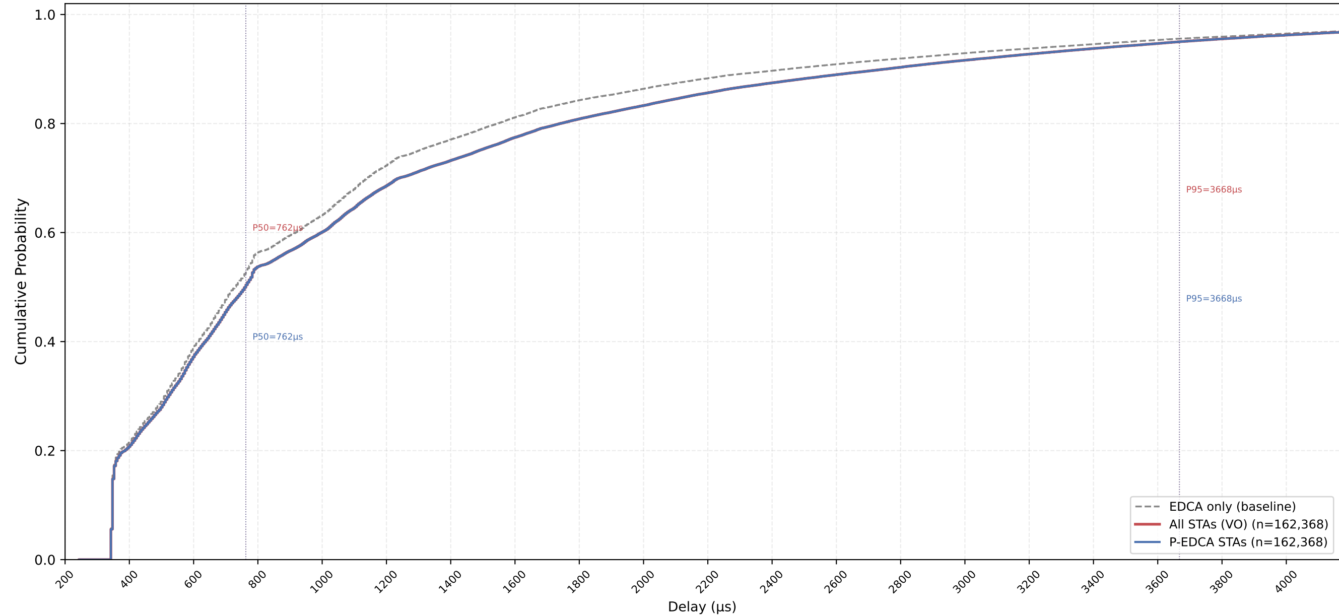
VO Delay CDF — P-EDCA / Legacy / All | CWds=0 × QSRC=2 × PSRC=2 nSta=30, nPedca=30/30, 0.5Mbps, avg of 10 runs
