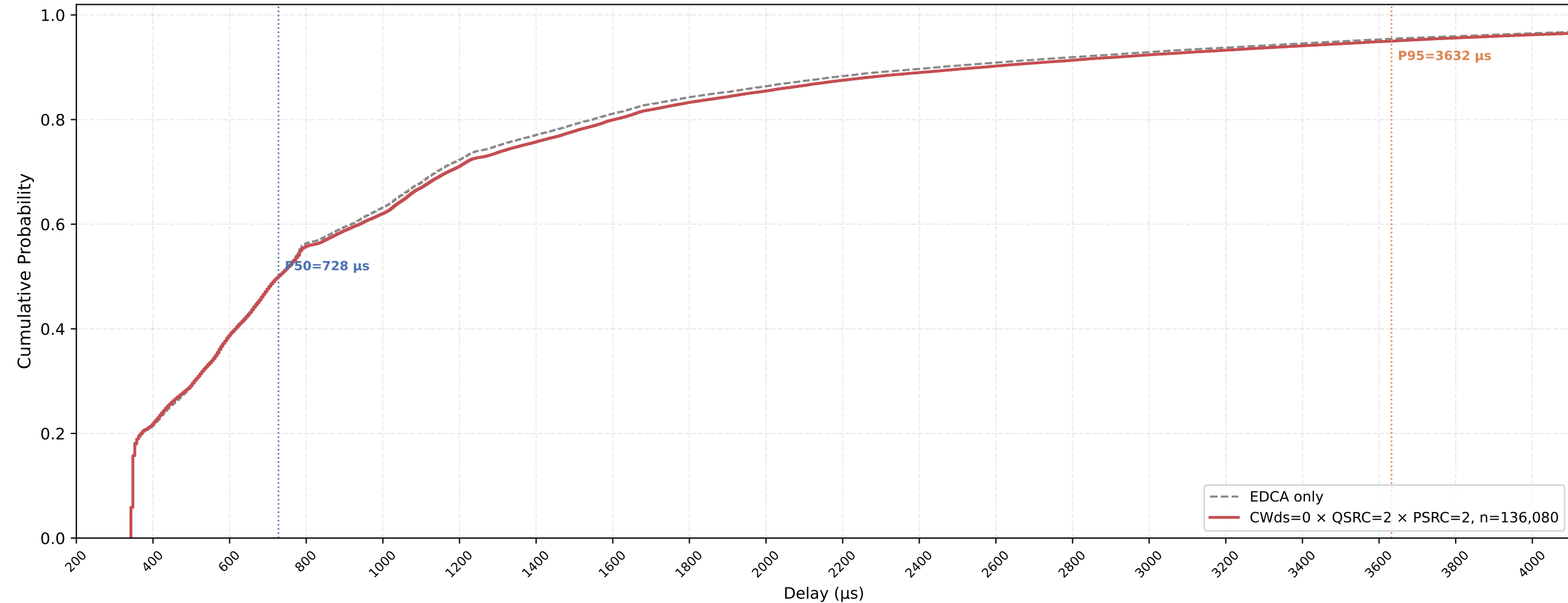
Legacy STA VO Delay CDF — CWds=0 × QSRC=2 × PSRC=2 nSta=30, nPedca=5, 0.5Mbps, avg of 10 runs
