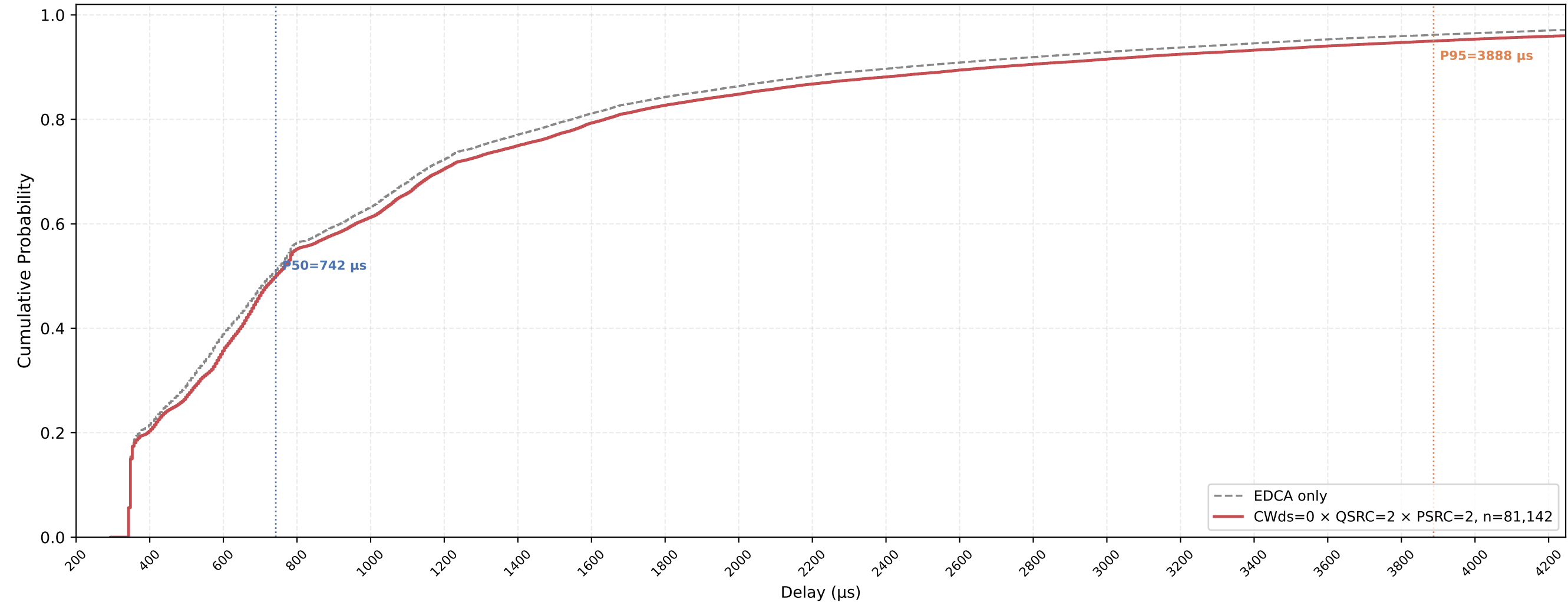
Legacy STA VO Delay CDF — CWds=0 × QSRC=2 × PSRC=2 nSta=30, nPedca=15, 0.5Mbps, avg of 10 runs
