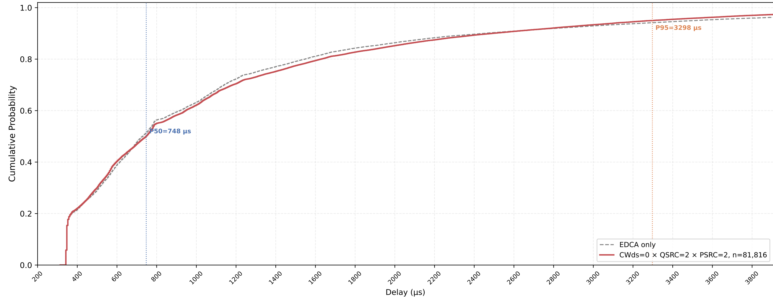
P-EDCA STA VO Delay CDF — CWds=0 × QSRC=2 × PSRC=2 nSta=30, nPedca=15, 0.5Mbps, avg of 10 runs
