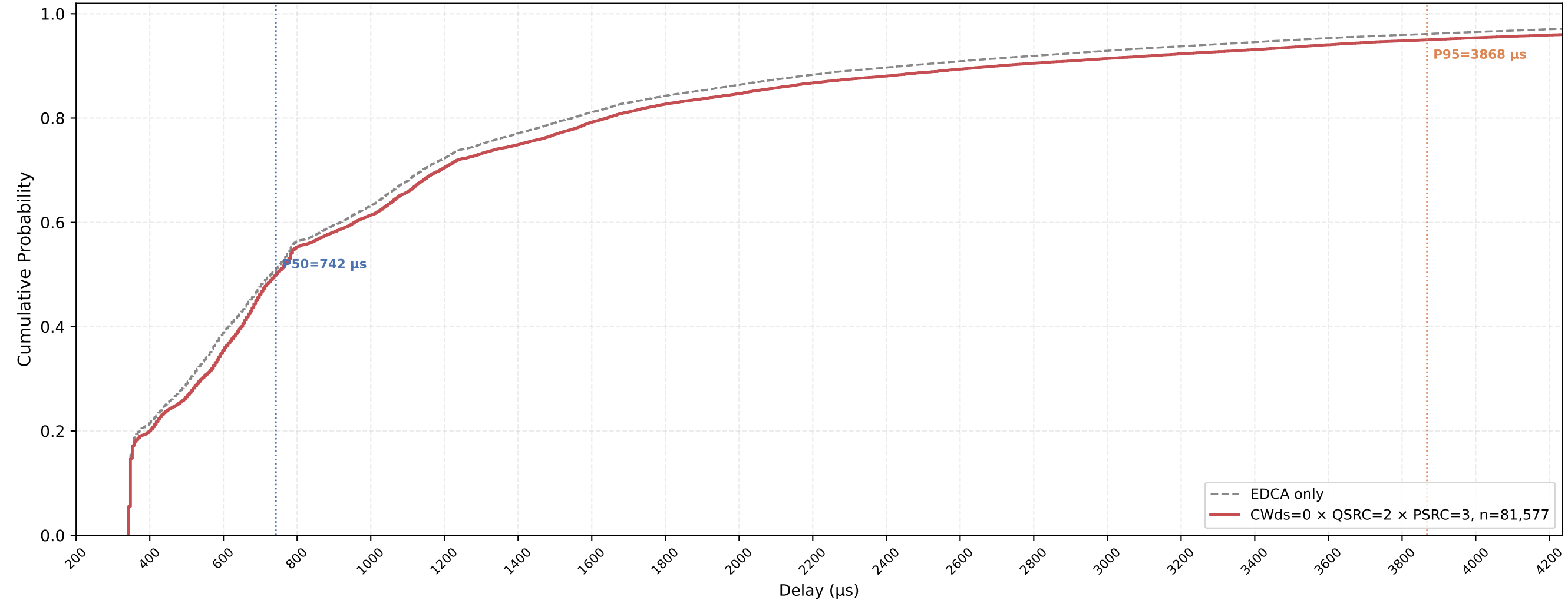
Legacy STA VO Delay CDF — CWds=0 × QSRC=2 × PSRC=3 nSta=30, nPedca=15, 0.5Mbps, avg of 10 runs
