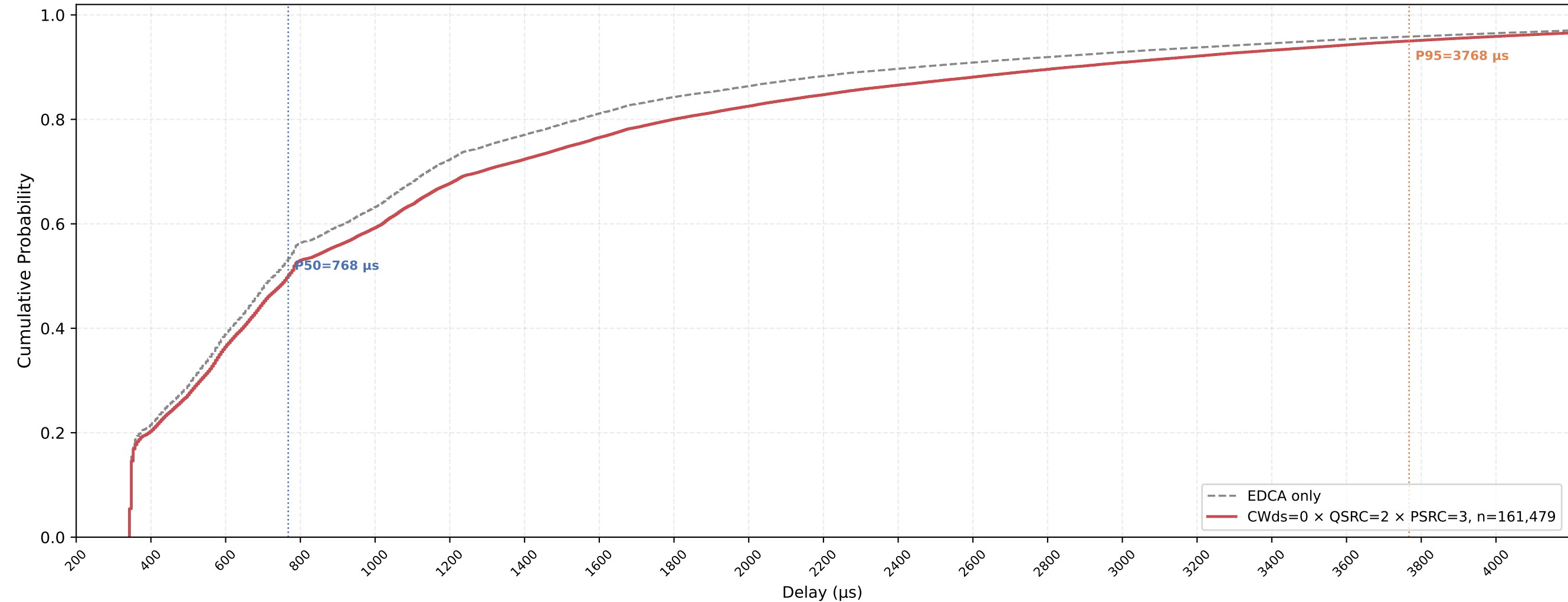
VO (all STAs) Delay CDF — CWds=0 × QSRC=2 × PSRC=3 nSta=30, nPedca=30, 0.5Mbps, avg of 10 runs
