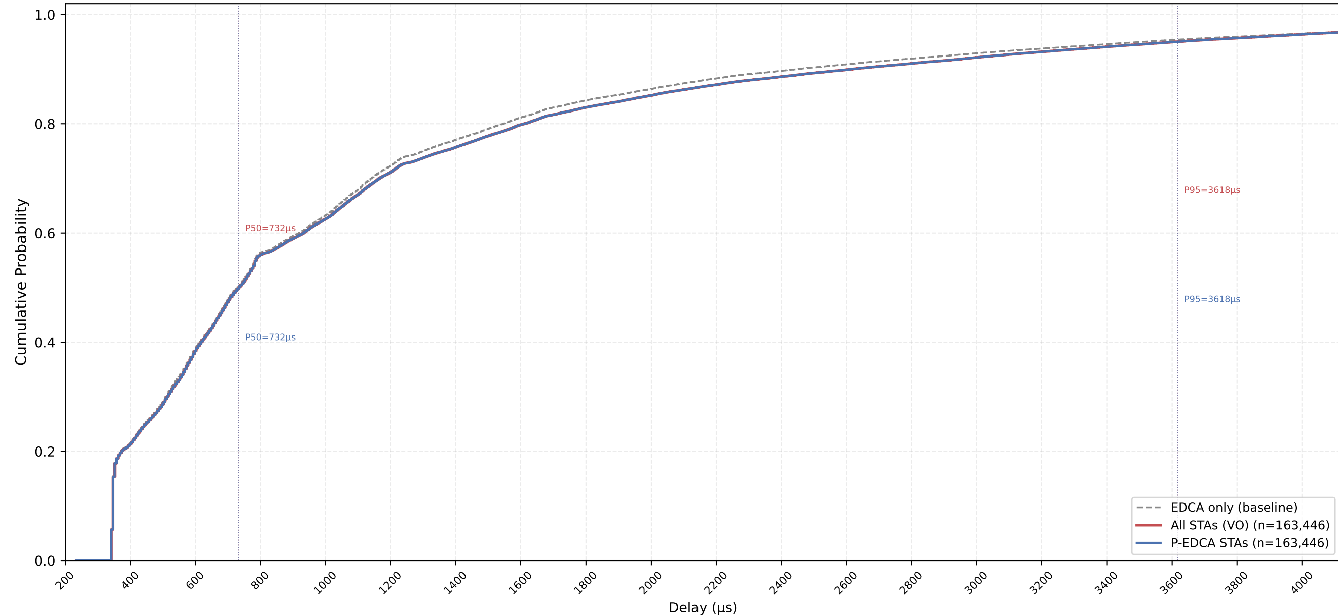
VO Delay CDF — P-EDCA / Legacy / All | CWds=0 × QSRC=3 × PSRC=1 nSta=30, nPedca=30/30, 0.5Mbps, avg of 10 runs
