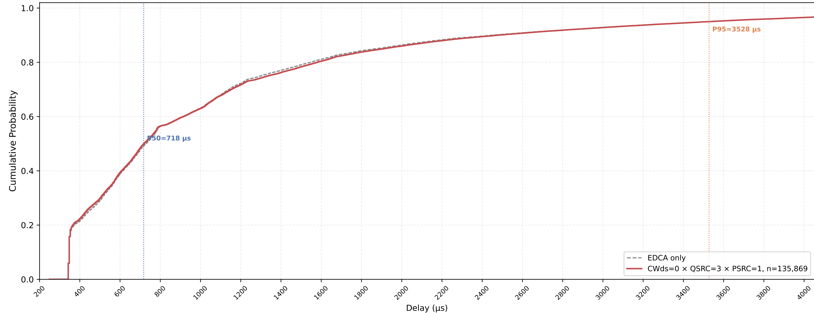
Legacy STA VO Delay CDF — CWds=0 × QSRC=3 × PSRC=1 nSta=30, nPedca=5, 0.5Mbps, avg of 10 runs
