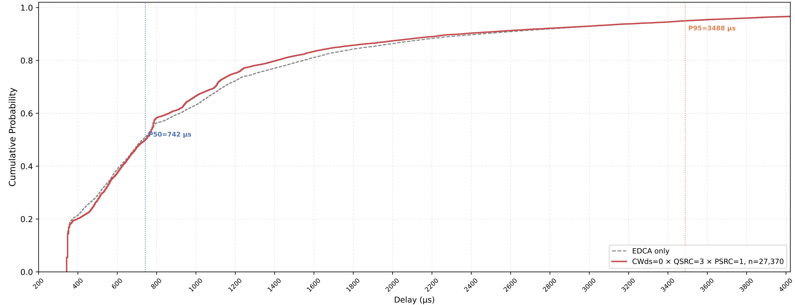
P-EDCA STA VO Delay CDF — CWds=0 × QSRC=3 × PSRC=1 nSta=30, nPedca=5, 0.5Mbps, avg of 10 runs
