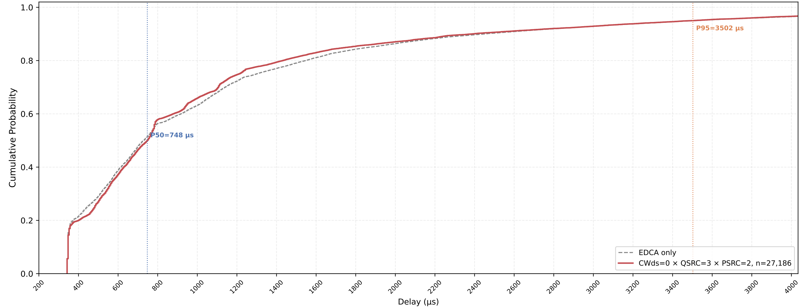
P-EDCA STA VO Delay CDF — CWds=0 × QSRC=3 × PSRC=2 nSta=30, nPedca=5, 0.5Mbps, avg of 10 runs
