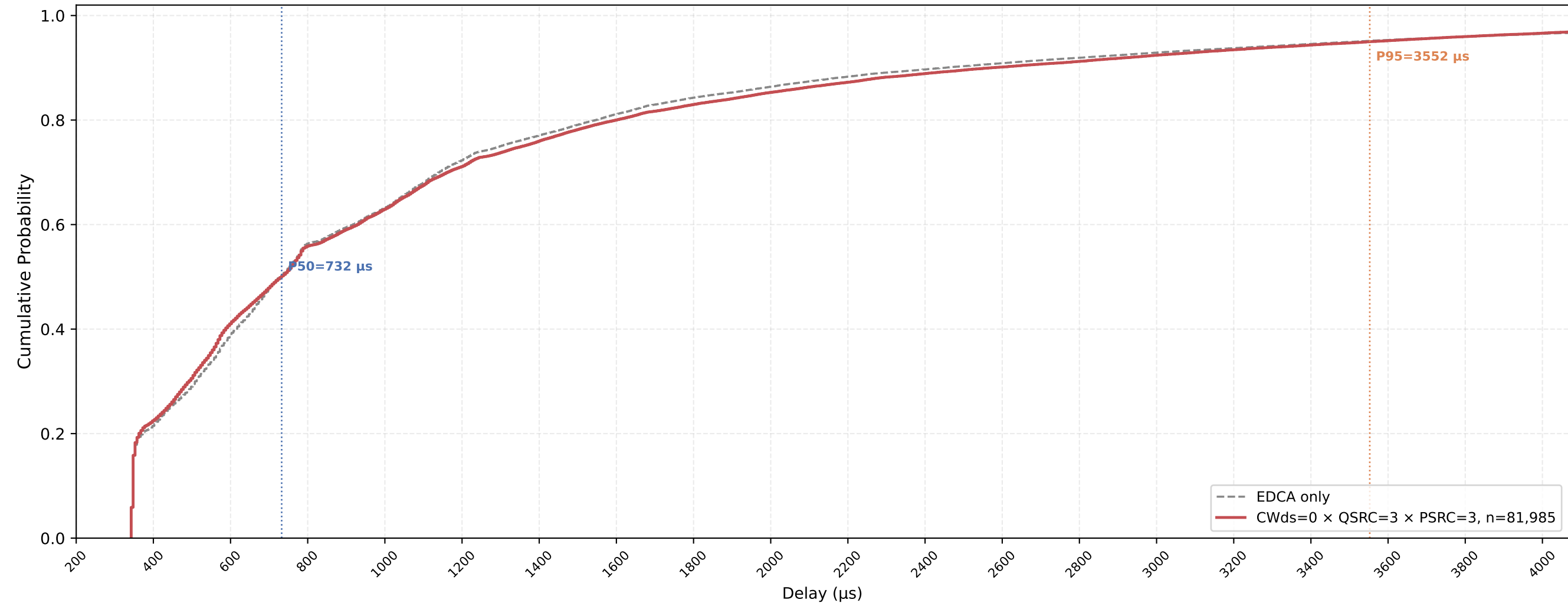
P-EDCA STA VO Delay CDF — CWds=0 × QSRC=3 × PSRC=3 nSta=30, nPedca=15, 0.5Mbps, avg of 10 runs
