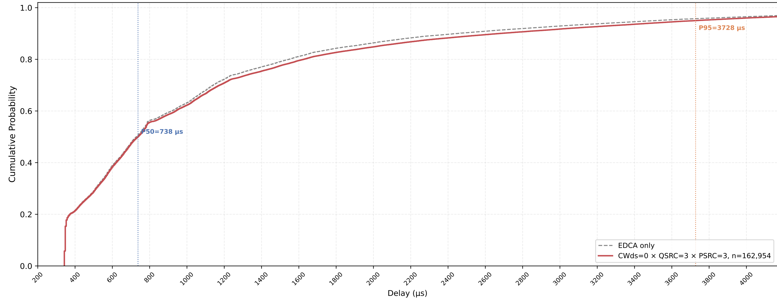
VO (all STAs) Delay CDF — CWds=0 × QSRC=3 × PSRC=3 nSta=30, nPedca=30, 0.5Mbps, avg of 10 runs
