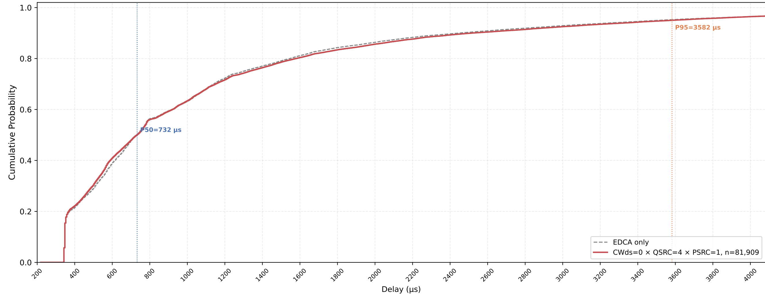
P-EDCA STA VO Delay CDF — CWds=0 × QSRC=4 × PSRC=1 nSta=30, nPedca=15, 0.5Mbps, avg of 10 runs
