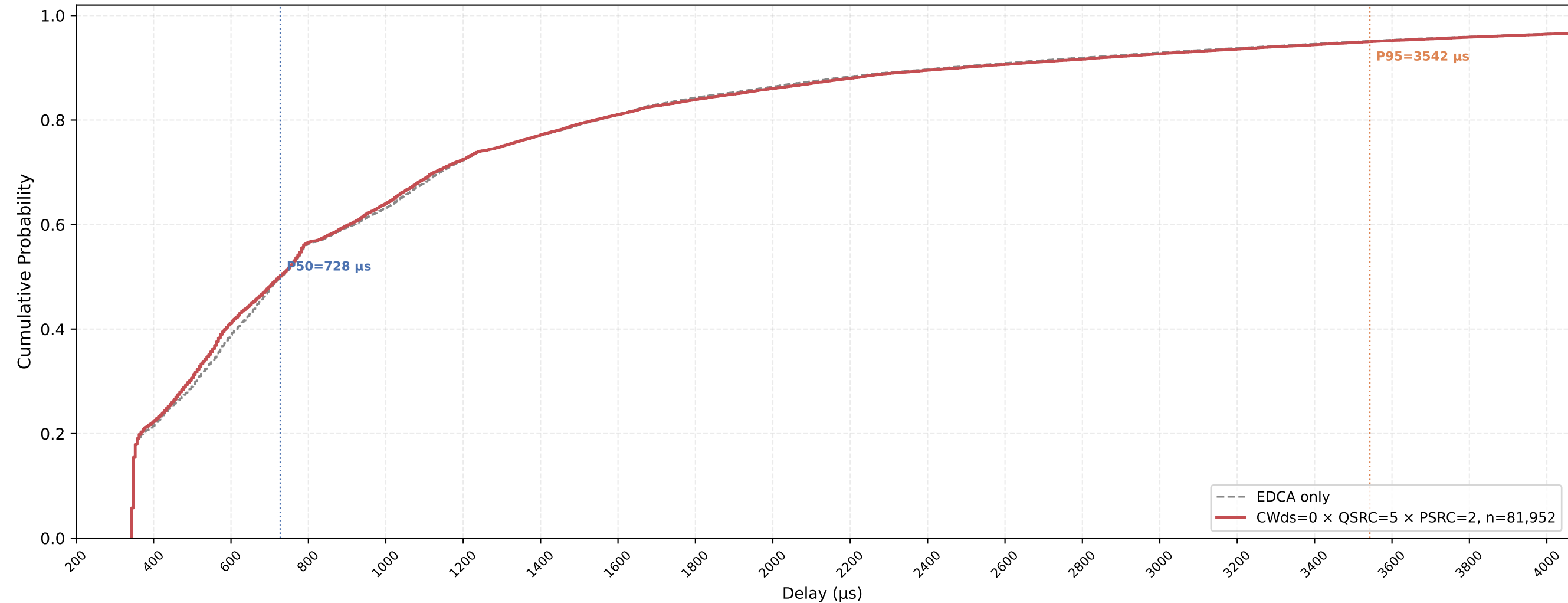
P-EDCA STA VO Delay CDF — CWds=0 × QSRC=5 × PSRC=2 nSta=30, nPedca=15, 0.5Mbps, avg of 10 runs
