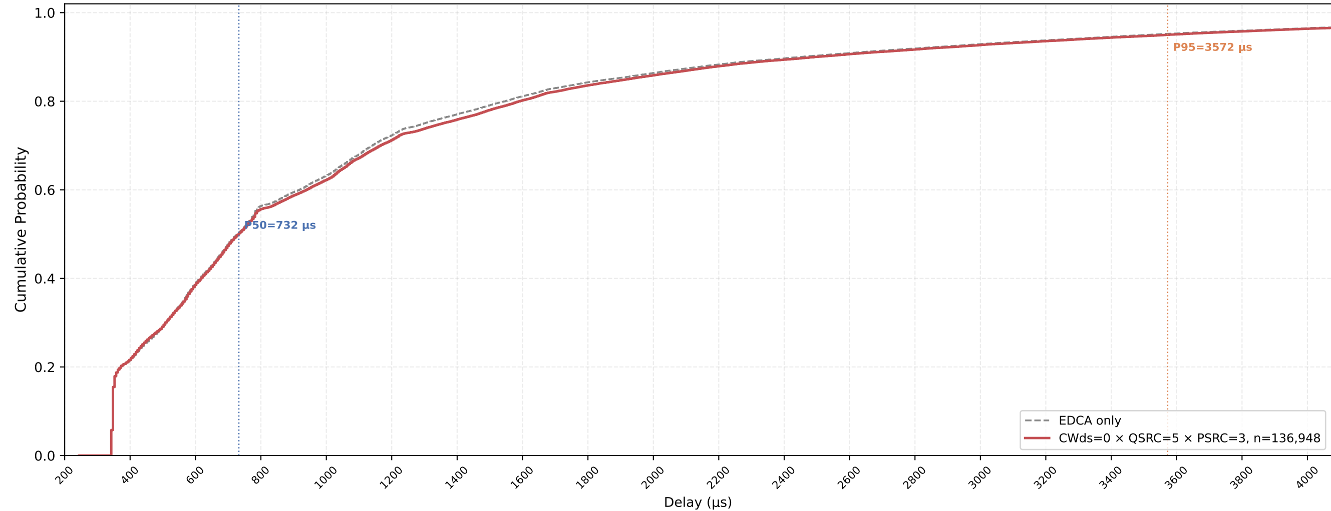
Legacy STA VO Delay CDF — CWds=0 × QSRC=5 × PSRC=3 nSta=30, nPedca=5, 0.5Mbps, avg of 10 runs
