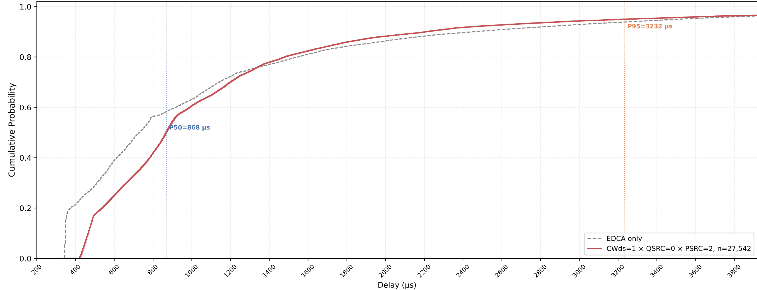
P-EDCA STA VO Delay CDF — CWds=1 × QSRC=0 × PSRC=2 nSta=30, nPedca=5, 0.5Mbps, avg of 10 runs
