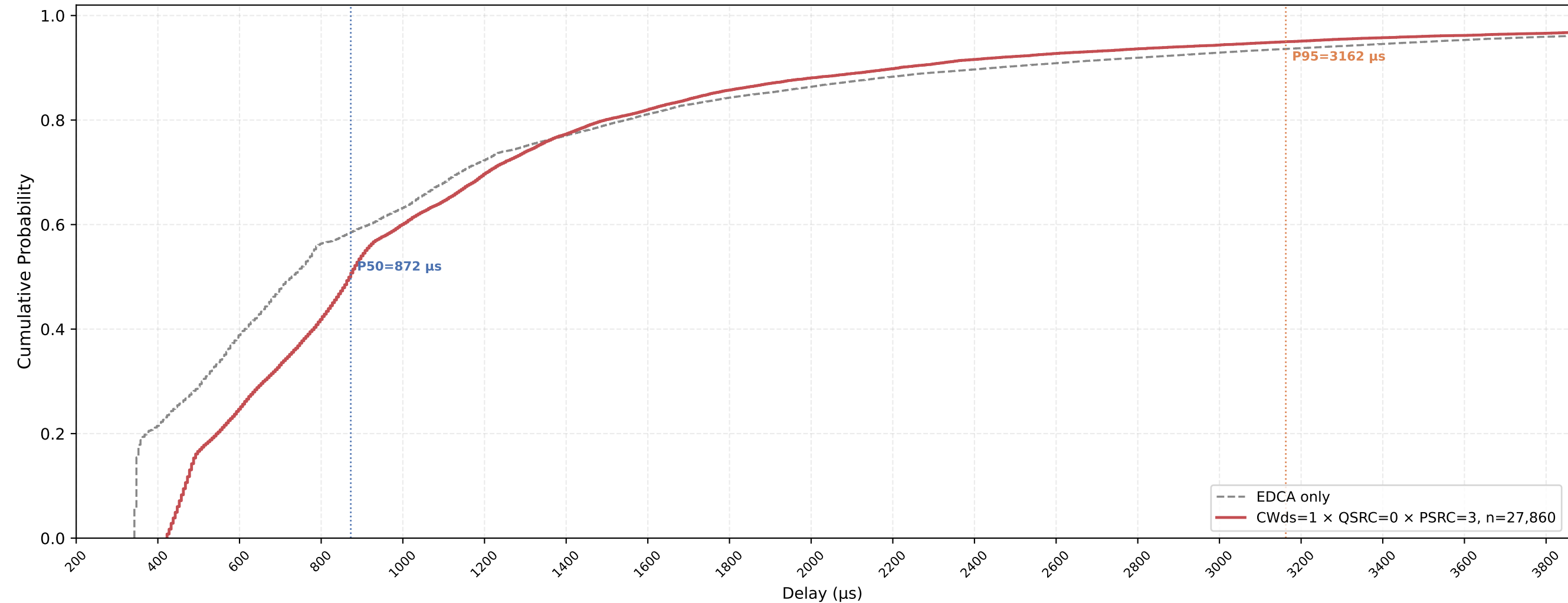
P-EDCA STA VO Delay CDF — CWds=1 × QSRC=0 × PSRC=3 nSta=30, nPedca=5, 0.5Mbps, avg of 10 runs
