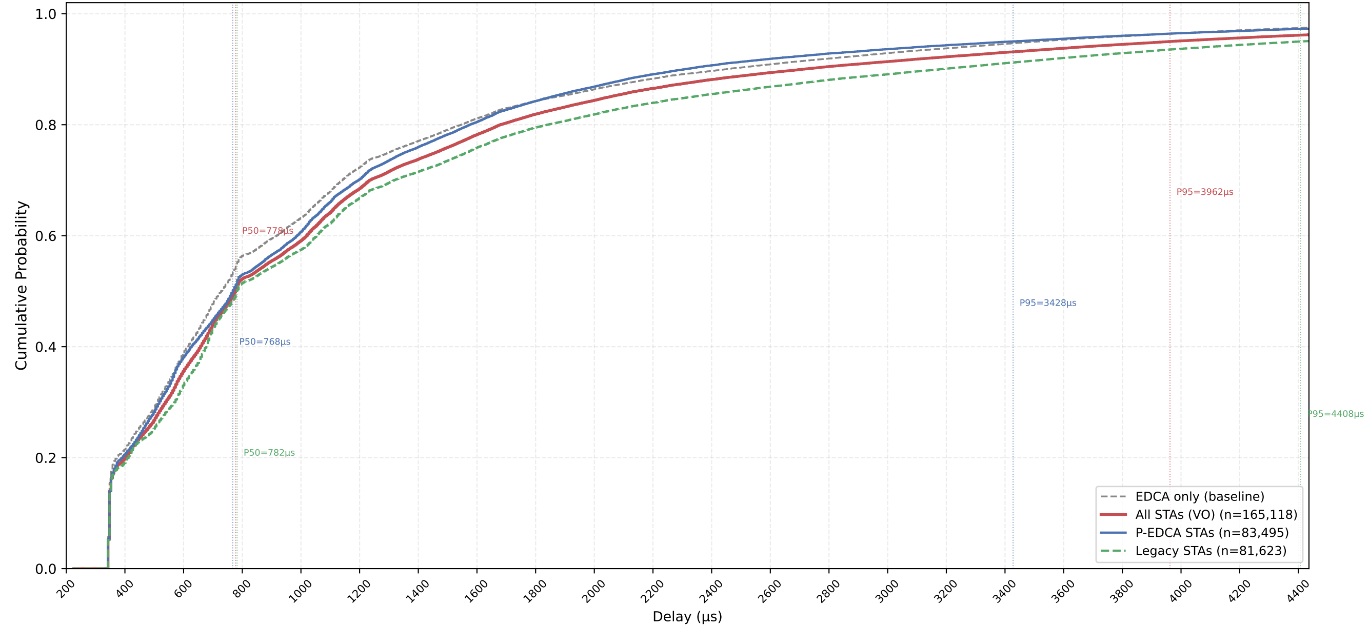
VO Delay CDF — P-EDCA / Legacy / All | CWds=1 × QSRC=1 × PSRC=2 nSta=30, nPedca=15/30, 0.5Mbps, avg of 10 runs
