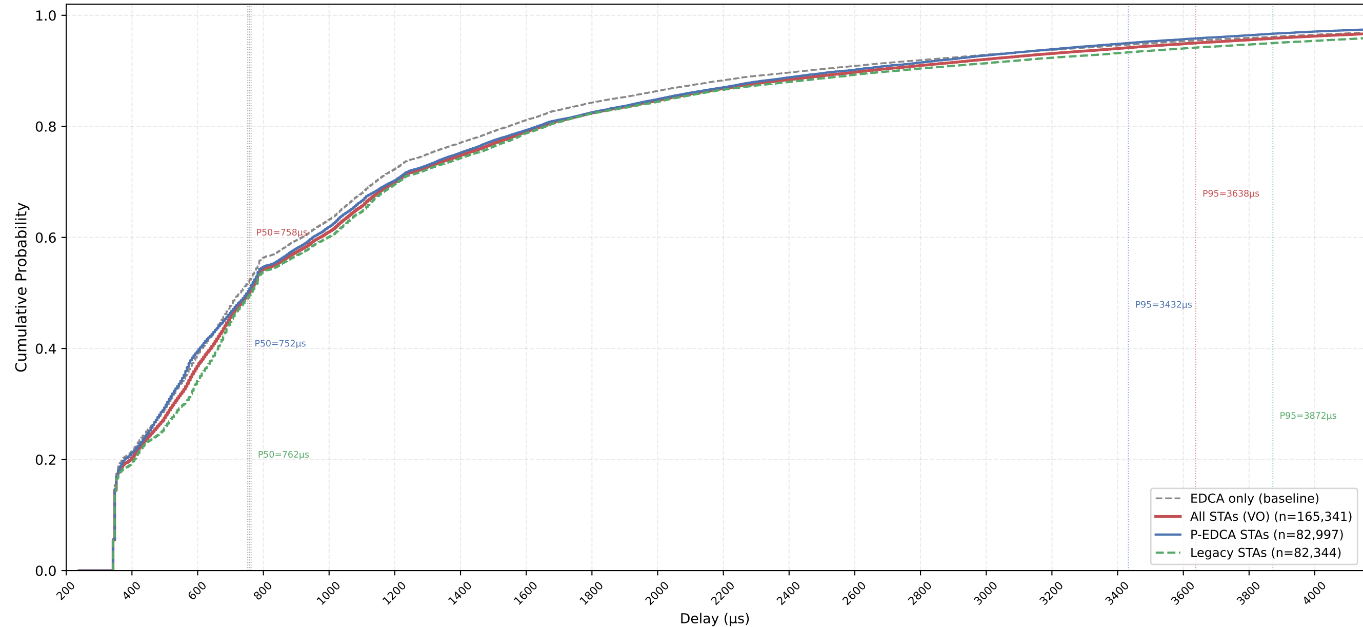
VO Delay CDF — P-EDCA / Legacy / All | CWds=1 × QSRC=2 × PSRC=2 nSta=30, nPedca=15/30, 0.5Mbps, avg of 10 runs
