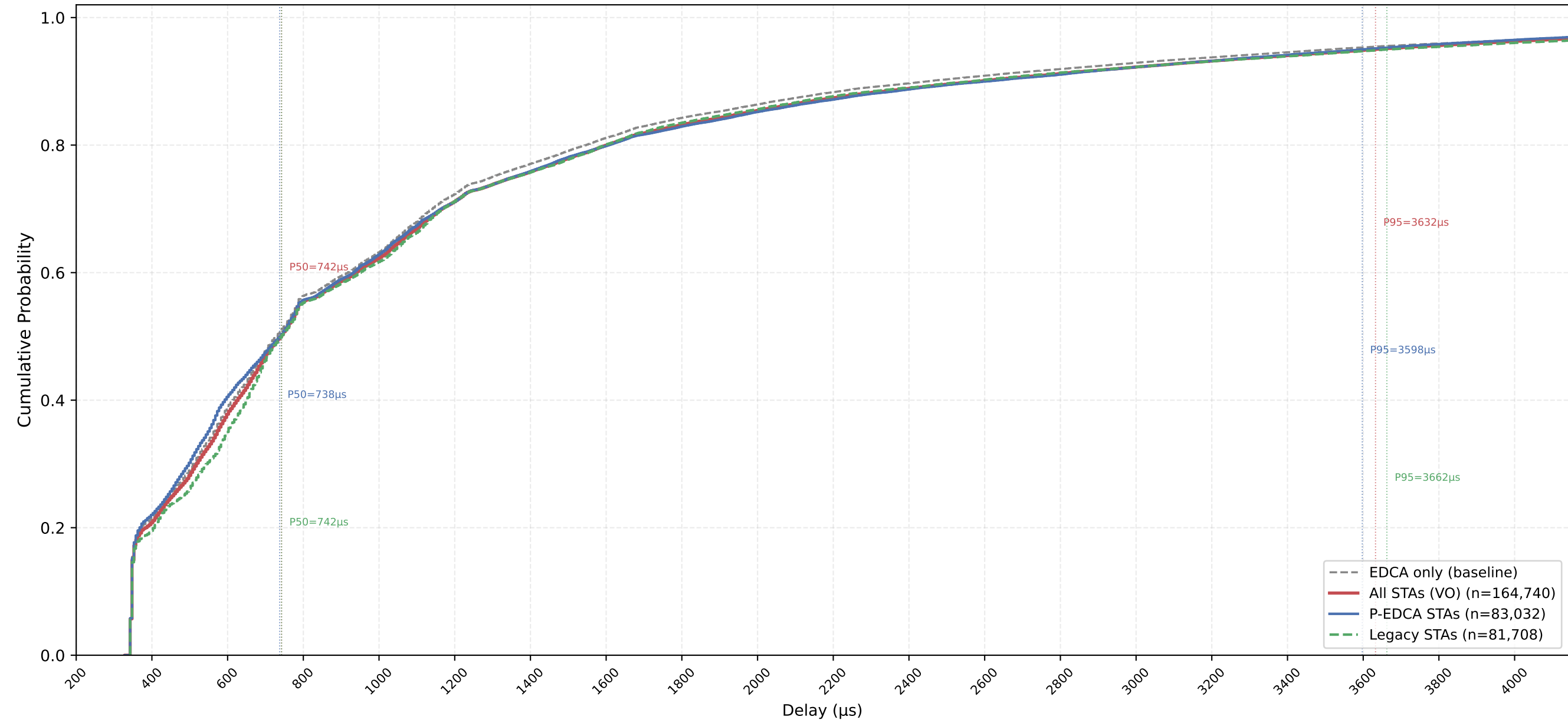
VO Delay CDF — P-EDCA / Legacy / All | CWds=1 × QSRC=3 × PSRC=2 nSta=30, nPedca=15/30, 0.5Mbps, avg of 10 runs
