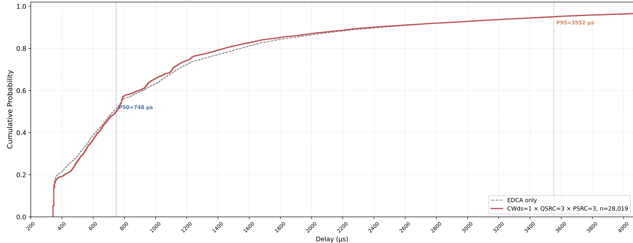
P-EDCA STA VO Delay CDF — CWds=1 × QSRC=3 × PSRC=3 nSta=30, nPedca=5, 0.5Mbps, avg of 10 runs
