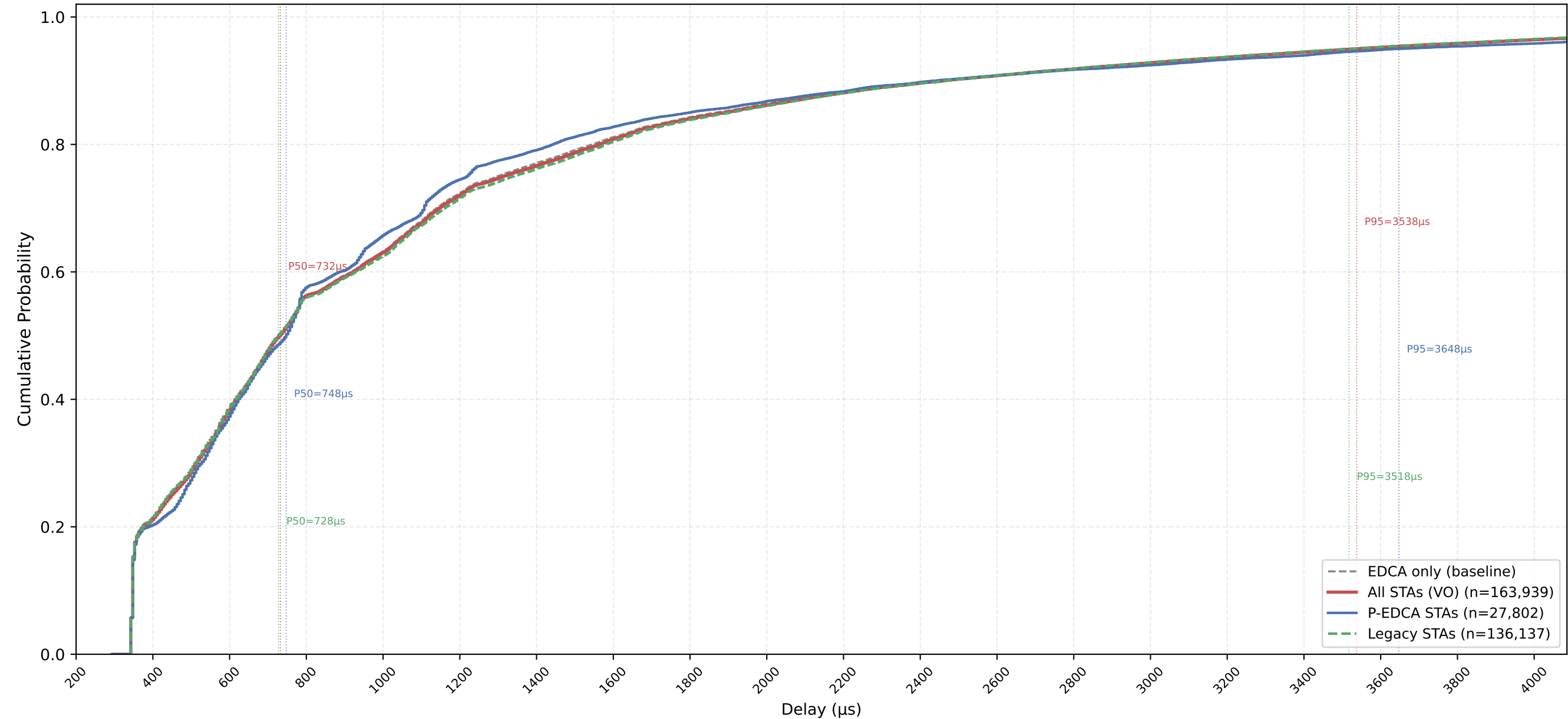
VO Delay CDF — P-EDCA / Legacy / All | CWds=1 × QSRC=4 × PSRC=1 nSta=30, nPedca=5/30, 0.5Mbps, avg of 10 runs
