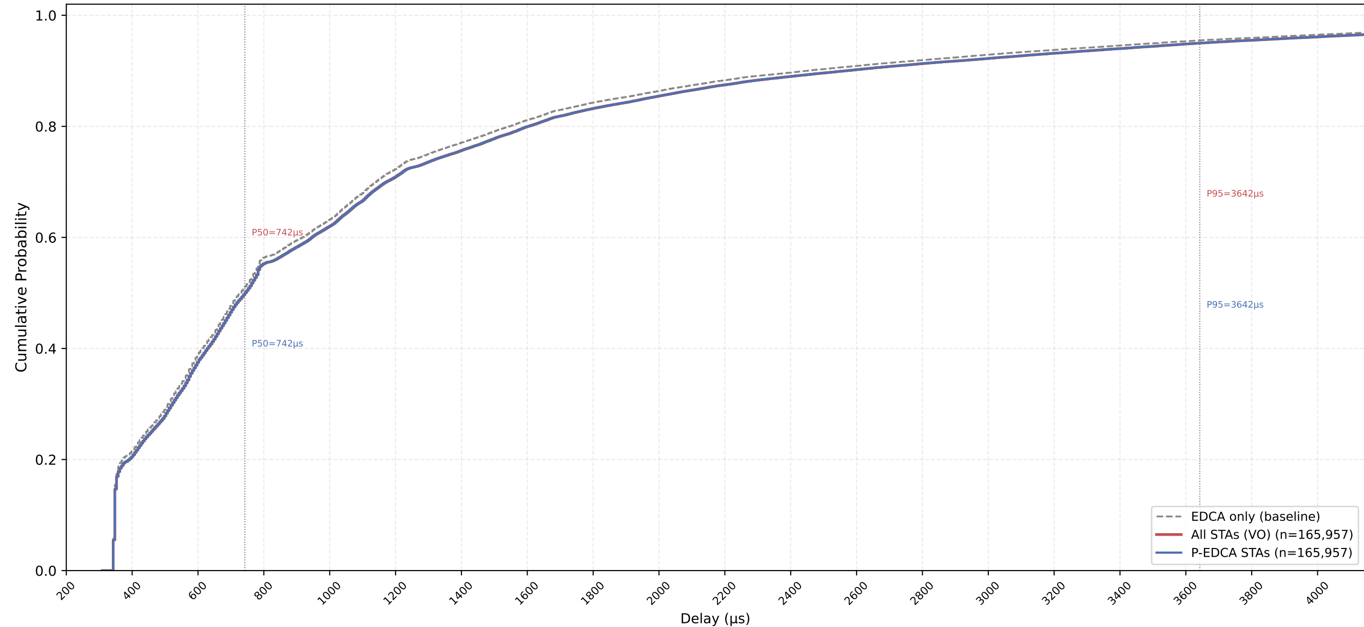
VO Delay CDF — P-EDCA / Legacy / All | CWds=1 × QSRC=4 × PSRC=2 nSta=30, nPedca=30/30, 0.5Mbps, avg of 10 runs
