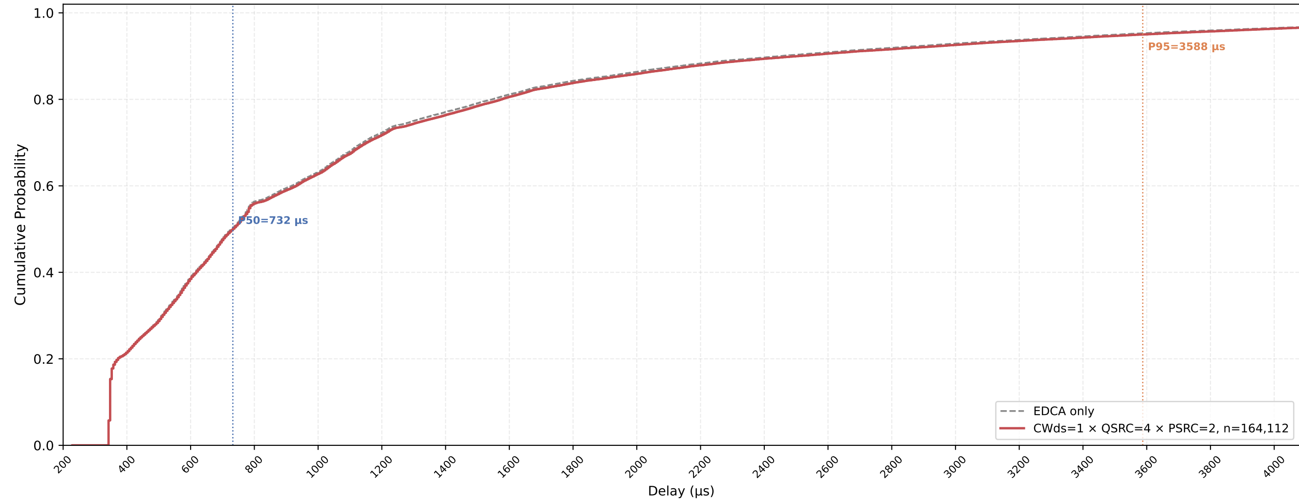
VO (all STAs) Delay CDF — CWds=1 × QSRC=4 × PSRC=2 nSta=30, nPedca=5, 0.5Mbps, avg of 10 runs
