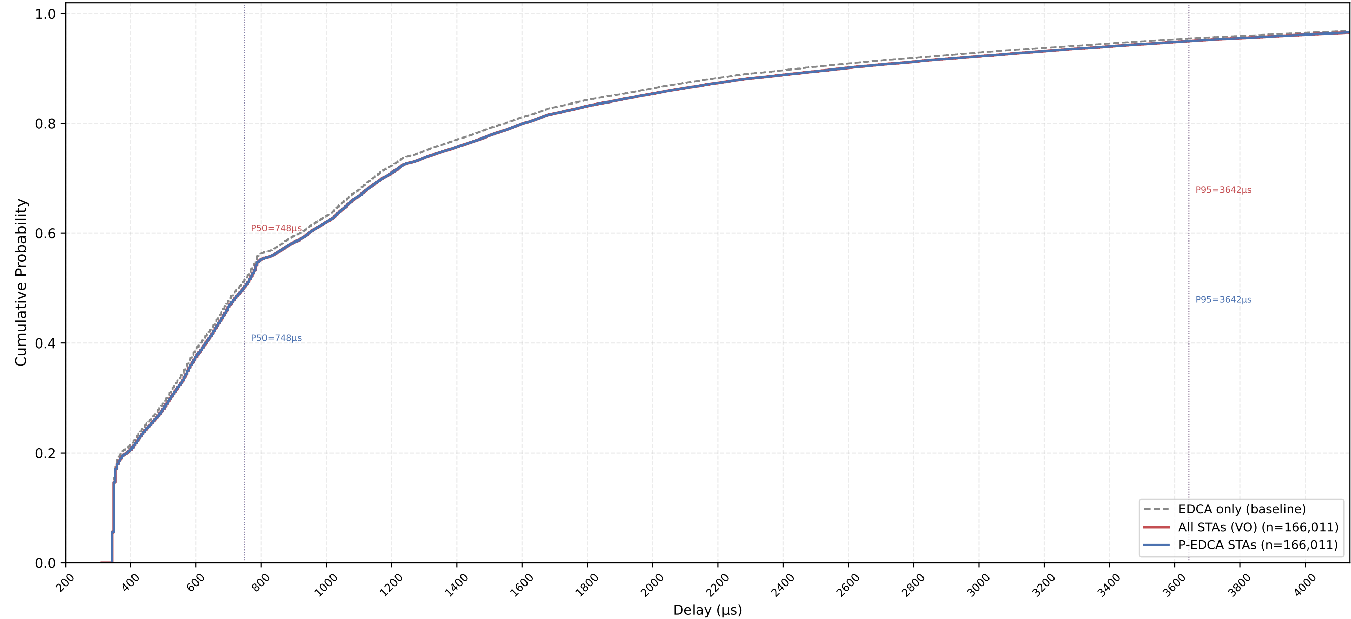
VO Delay CDF — P-EDCA / Legacy / All | CWds=1 × QSRC=4 × PSRC=3 nSta=30, nPedca=30/30, 0.5Mbps, avg of 10 runs
